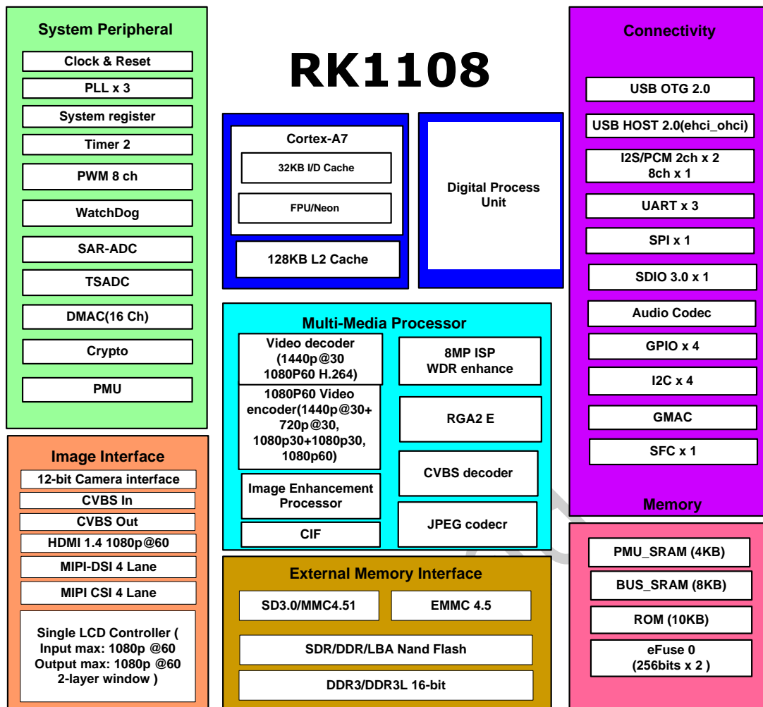
Fig. 1-1 RK1108 Block Diagram
