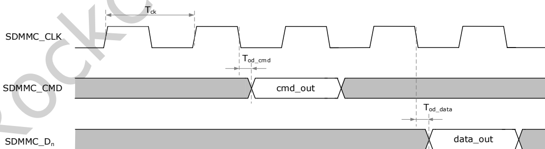
Fig. 4-4 SDMMC High Speed Mode Output Timing
