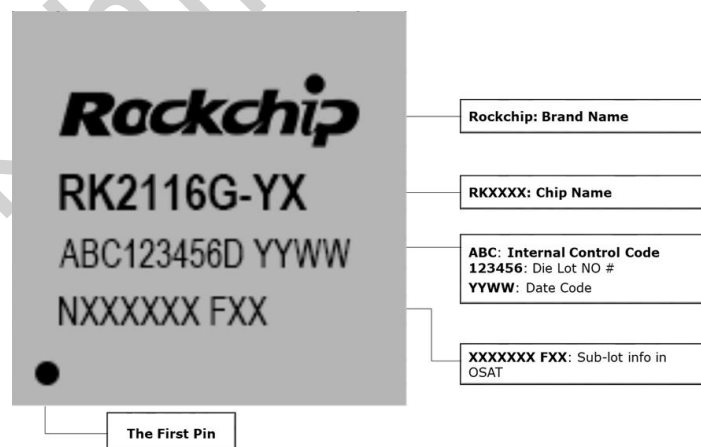
Fig.2-2 RK2116G-YX Package Definition
