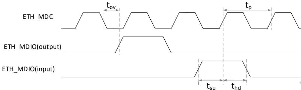
Fig. 4-7 MDIO Timing Diagram
