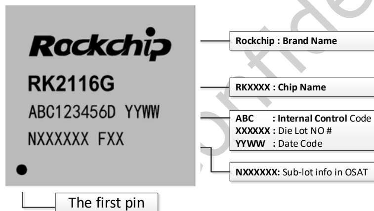
Fig.2-1 RK2116G Package Definition
