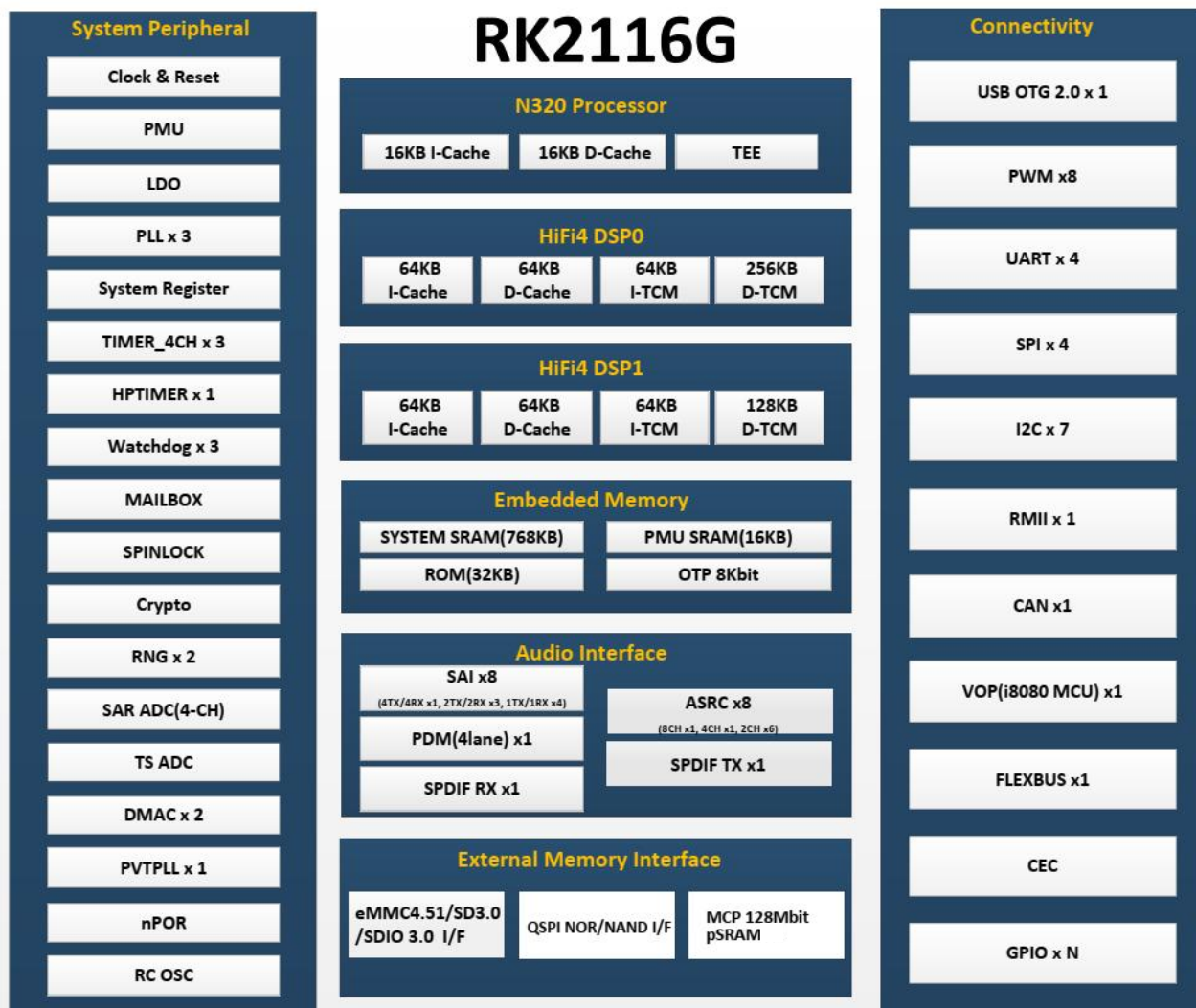
Fig.1-1 RK2116G Block Diagram
