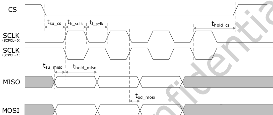
Fig. 4-11 SPI Master Mode Timing Diagram
