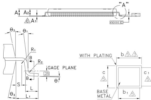
Fig.2-6 RK2116G Package Side View
