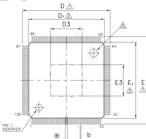
Fig.2-5 RK2116G Package Top View
