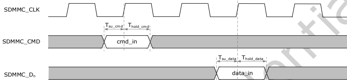
Fig. 4-3 SDMMC Default Speed Mode Input Timing
