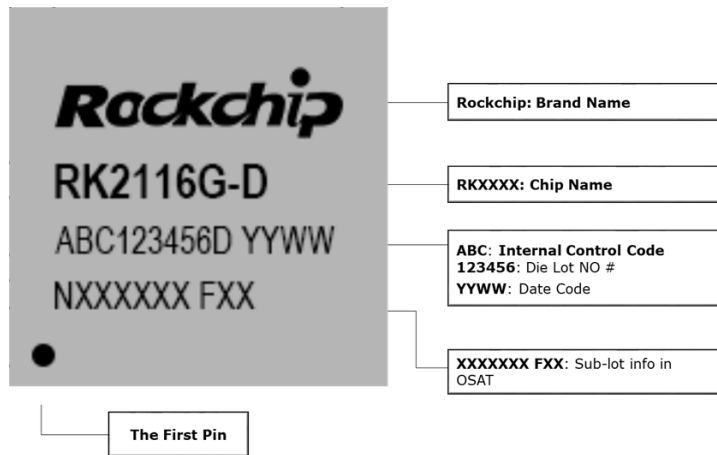
Fig.2-4 RK2116G-D Package Definition
