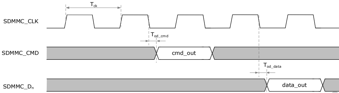
Fig. 4-2 SDMMC Default Speed Mode Output Timing
