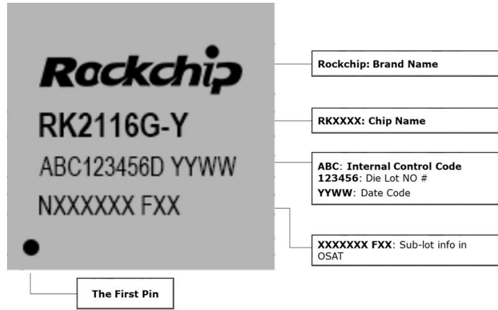
Fig.2-3 RK2116G-Y Package Definition
