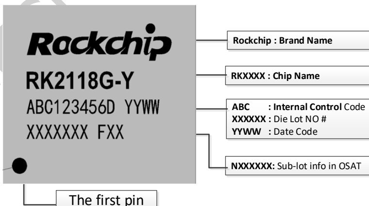
Fig.2-2 RK2118G-Y Package Definition
