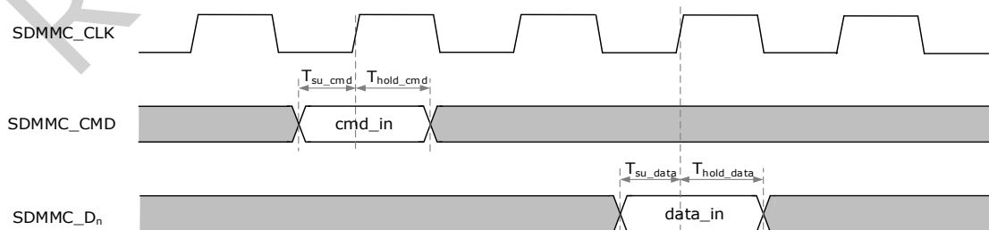
Fig. 4-9 SDMMC Default Speed Mode Input Timing
