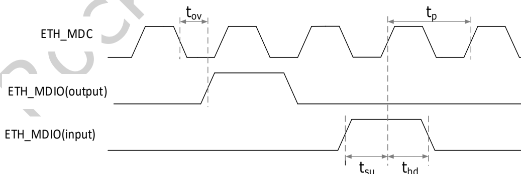
Fig. 4-13 MDIO Timing
