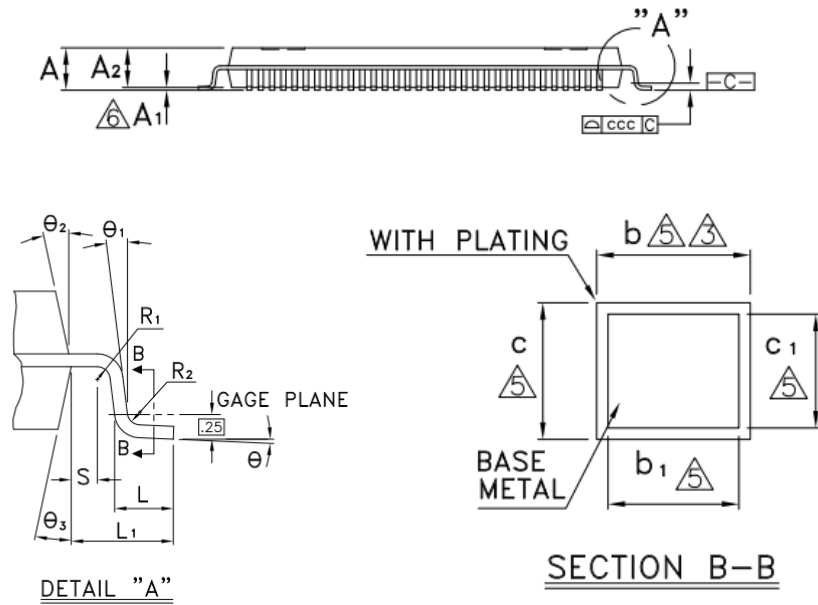
Fig.2-3 RK2118M Package Side View
