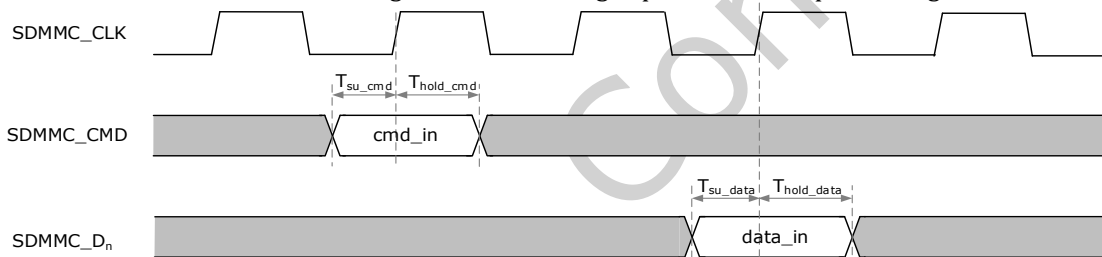
Fig. 4-11 SDMMC High Speed Mode Output Timing
