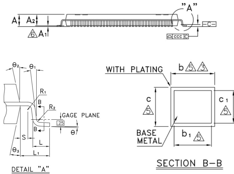
Fig.2-3 RK2118M Package Side View
