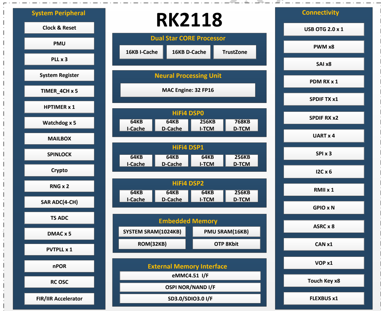
Fig.1-1 RK2118M Block Diagram
