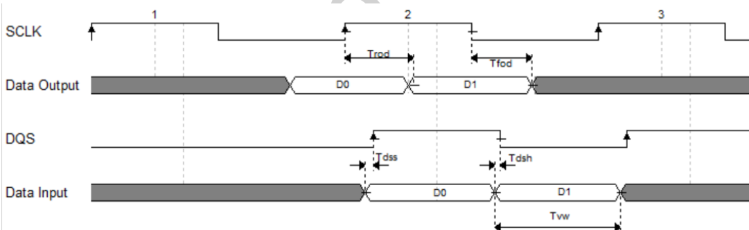
Fig. 4-2 FSPI SCLK and data timing diagram (DDR read with DQS mode and DDR write mode)
