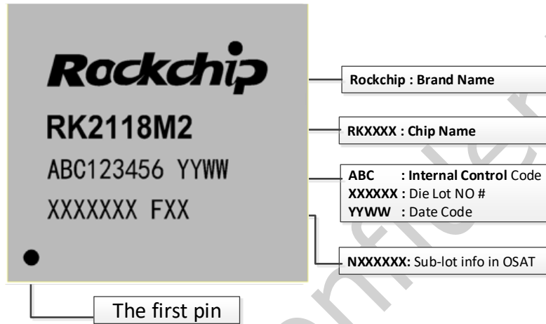
Fig.2-1 RK2118M2 Package Definition
