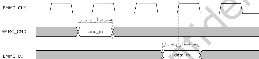
Fig. 4-5 eMMC Backward Mode input Timing
