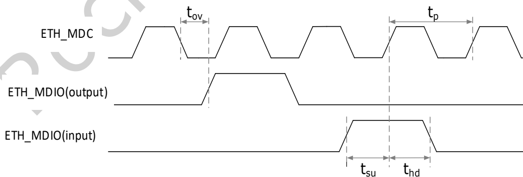
Fig. 4-13 MDIO Timing
