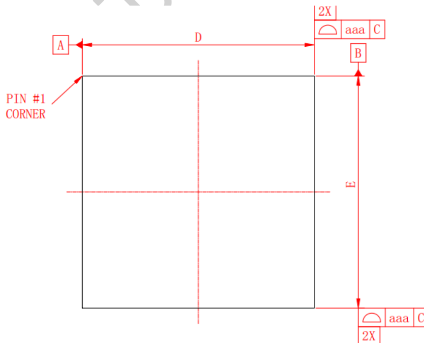
Fig.2-2 RK2118M2 Package Top View
