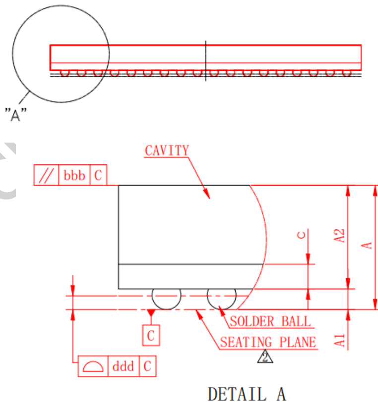
Fig.2-4 RK2118M2 Package Side View
