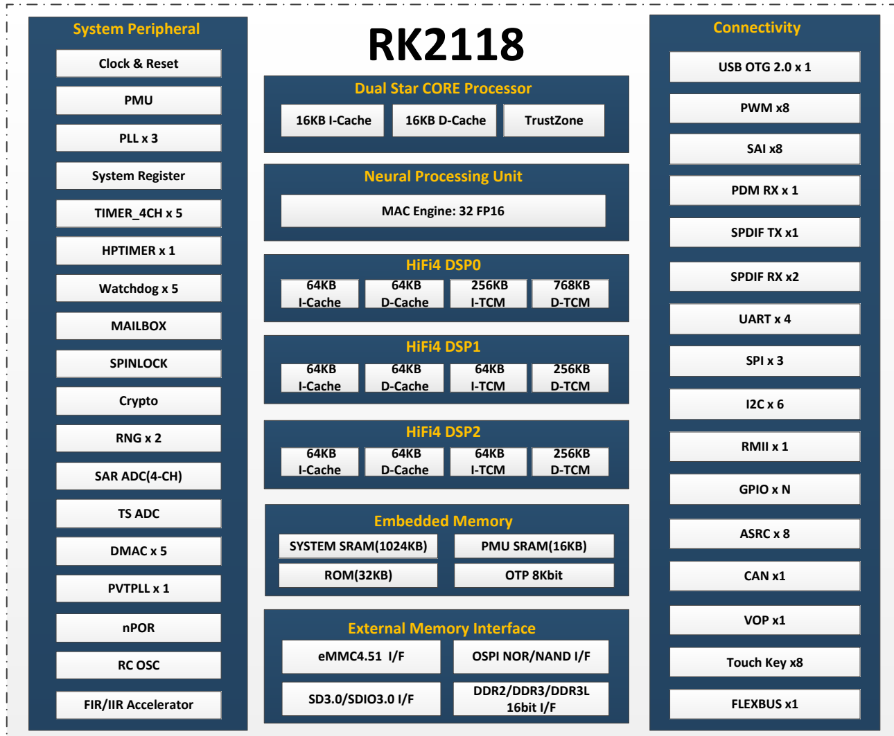
Fig.1-1 RK2118M2 Block Diagram
