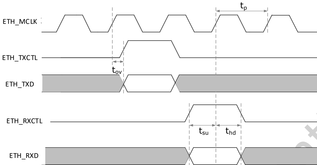
Fig. 4-12 RMII Interface Timing
