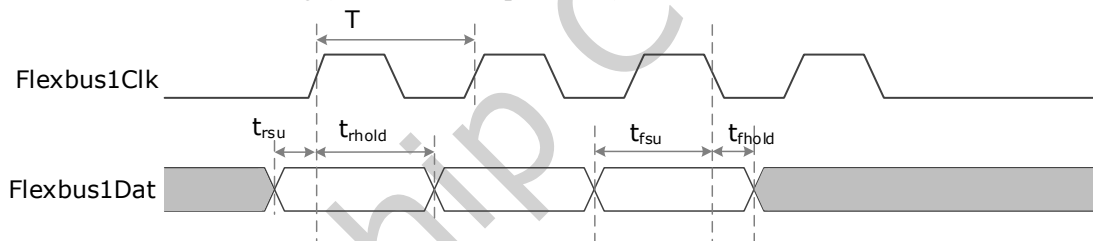
Fig. 4-22 Flexbus RX Timing Diagram 1 in Slave Mode
