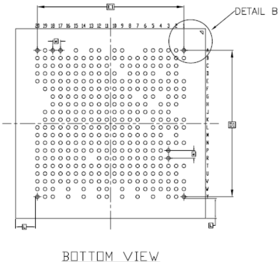
Fig.2-3 RK3308H3 Package bottom view
