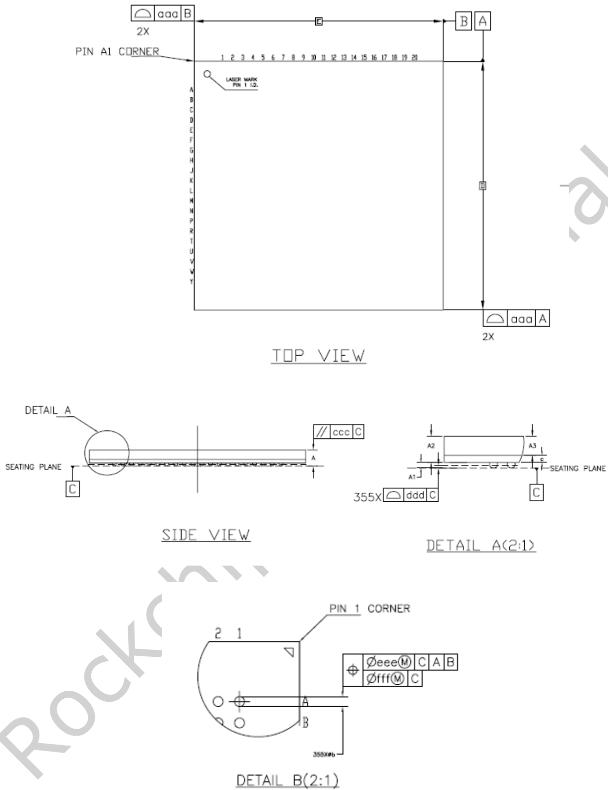
Fig.2-2 RK3308H3 Package Top View and Side View
