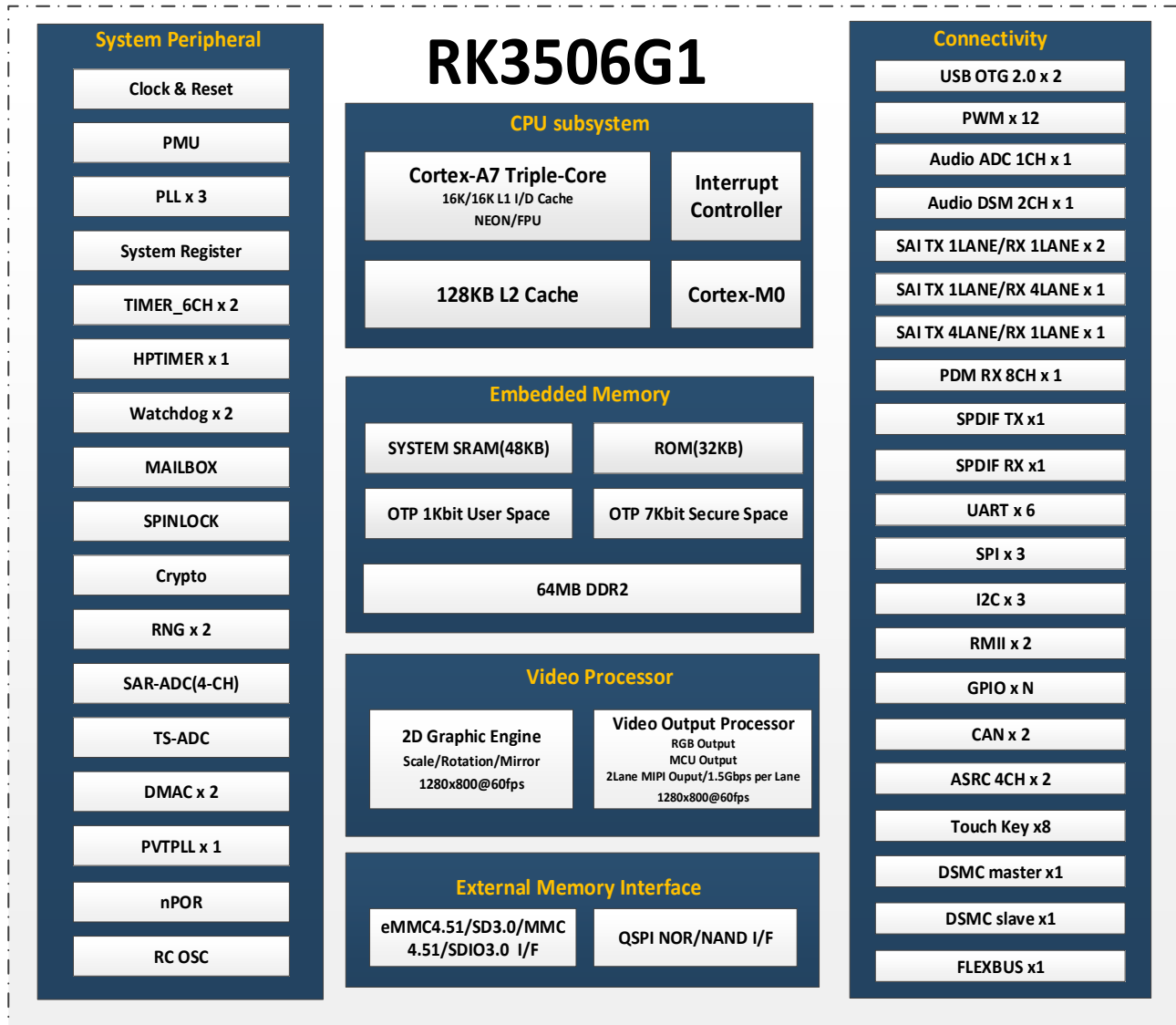
Fig.1-1 RK3506G1 Block Diagram
