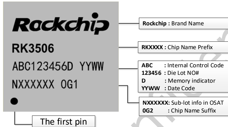
Fig.2-1 RK3506G1 Package Definition
