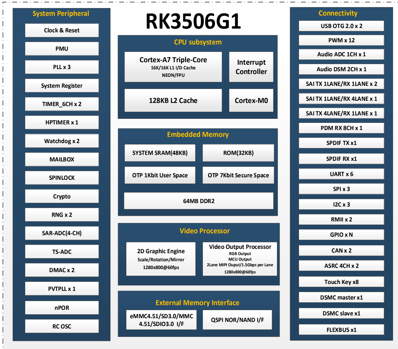
Fig.1-1 RK3506G1 Block Diagram
