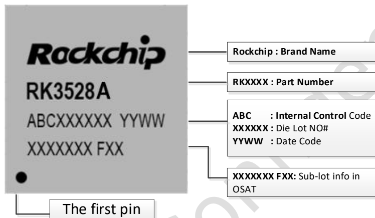
Fig.2-1 RK3528A Package definition
