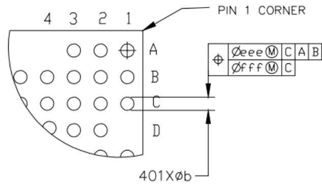
DETAIL B(2:1)
