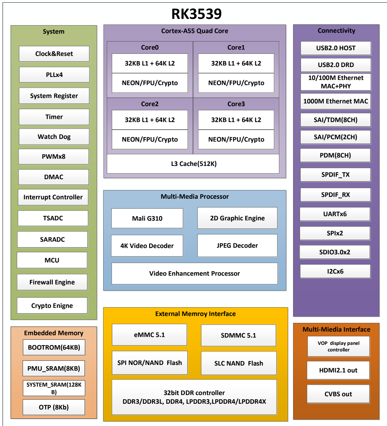
Fig.1-1 Block Diagram
