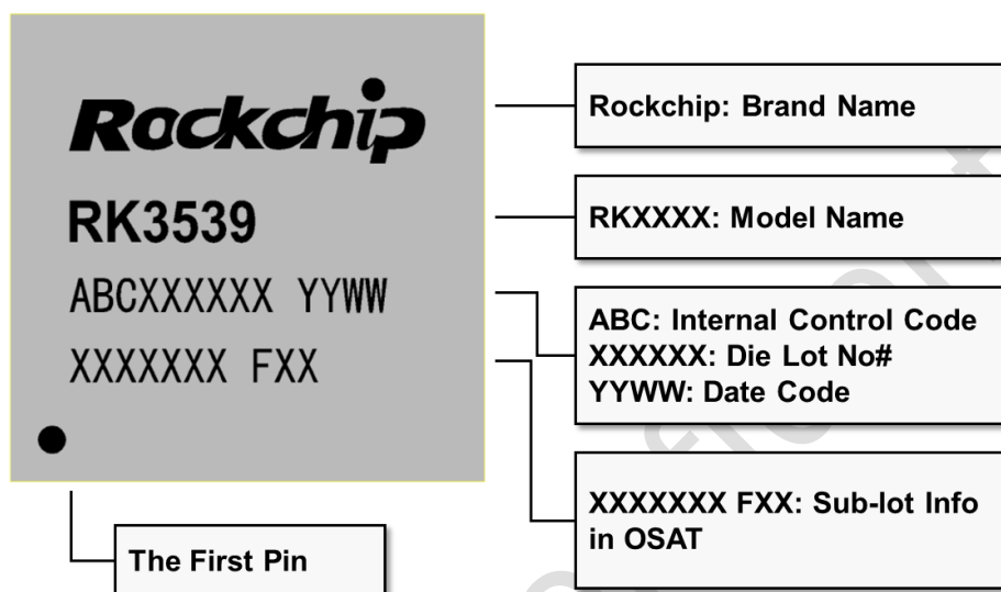
Fig.2-1 Package Definition
