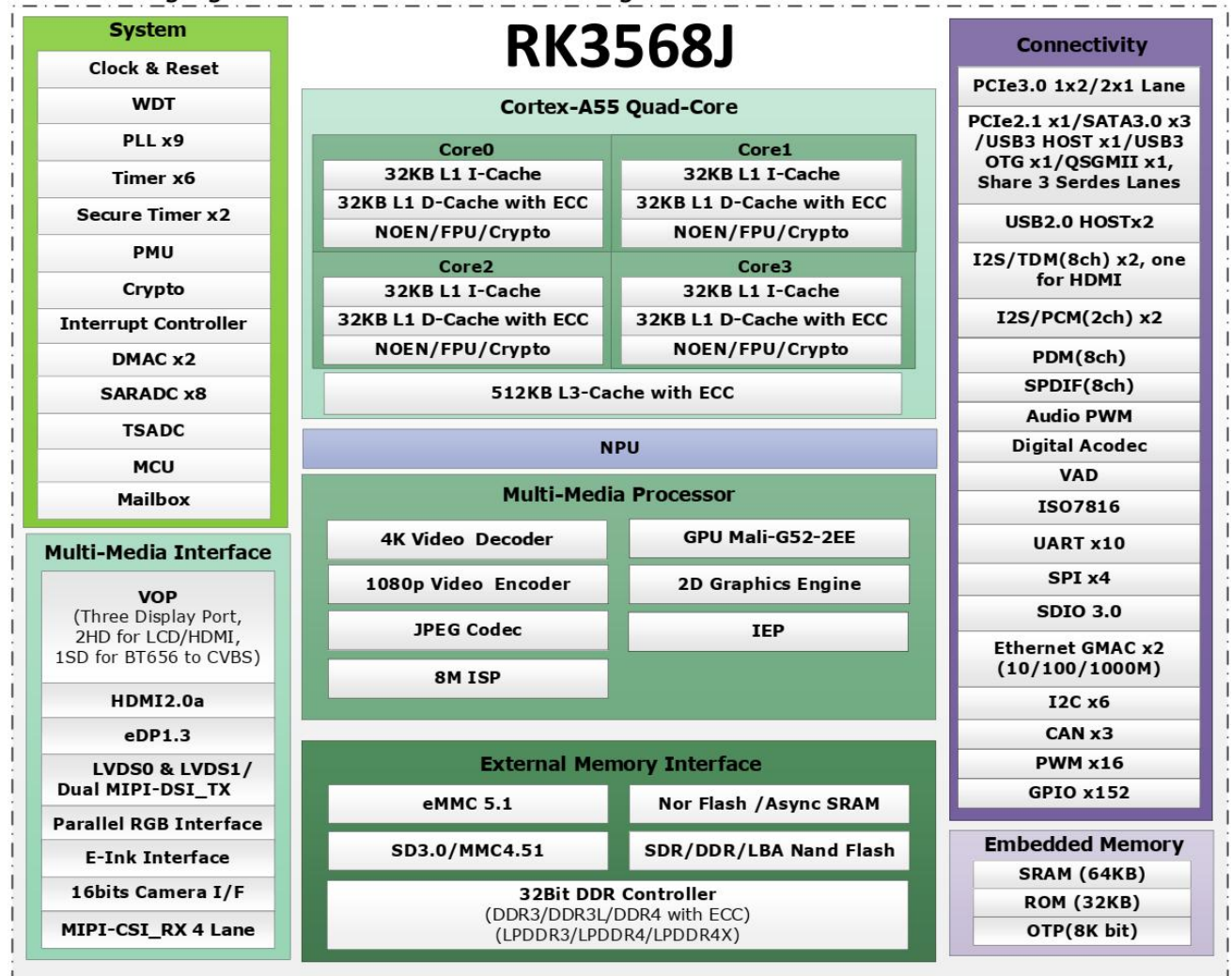
Fig.1-1 Block Diagram
