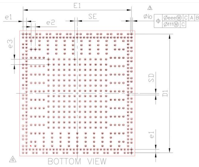
Fig. 2-3 Package Bottom View
