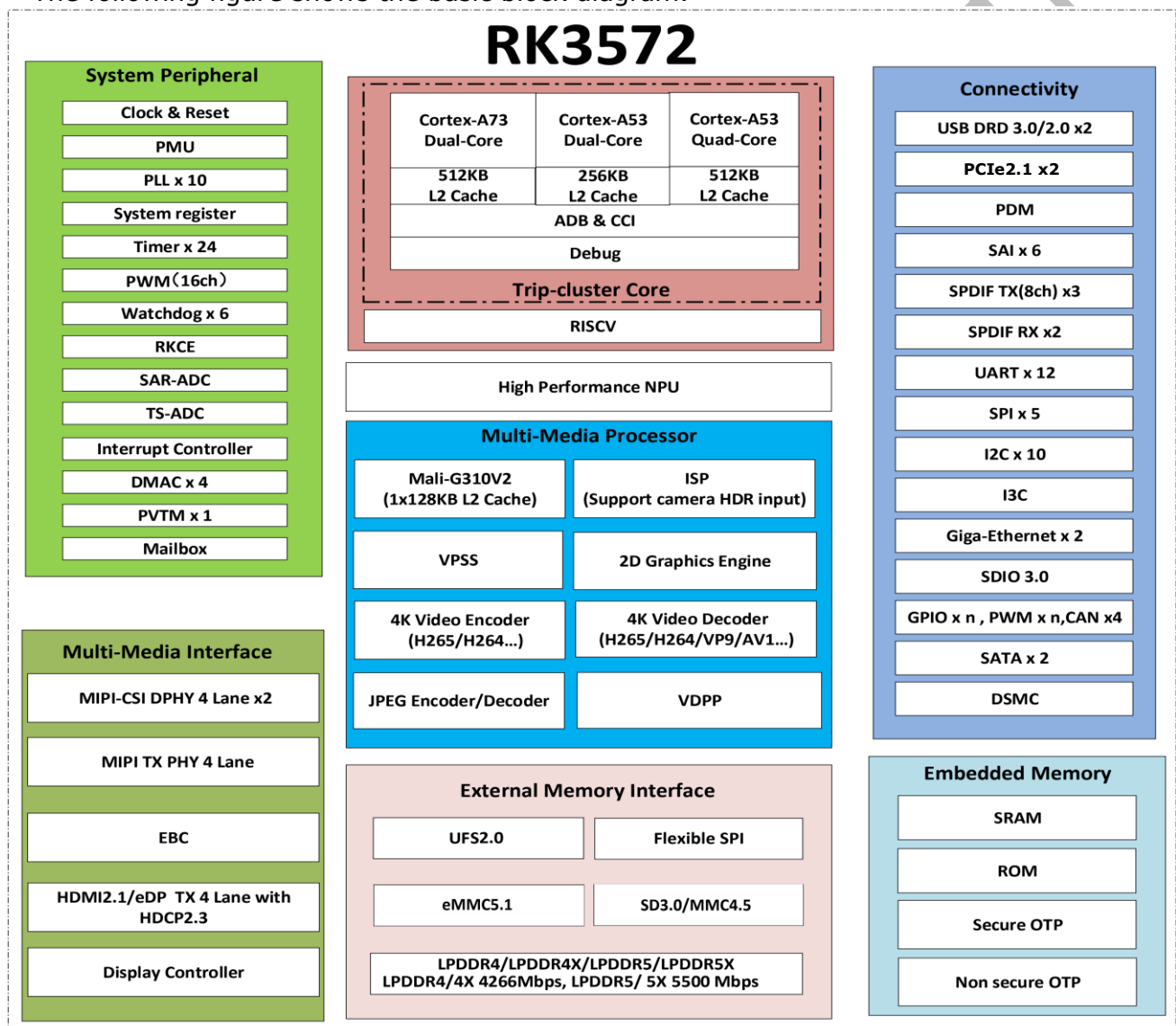
Fig. 1-1 Block Diagram
