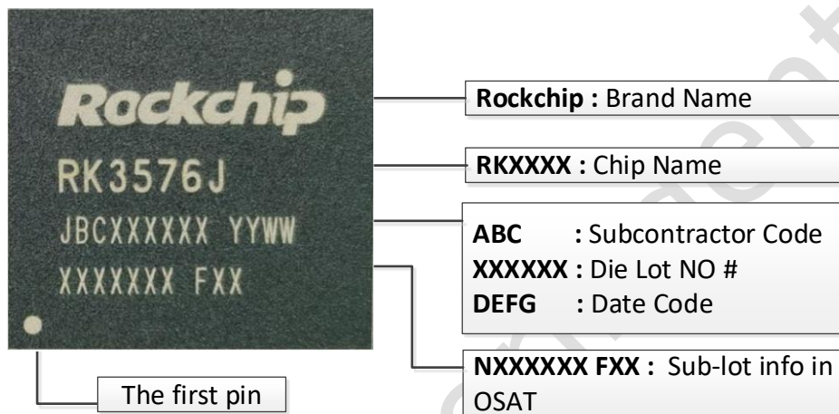
Fig.2-1 Package Definition
