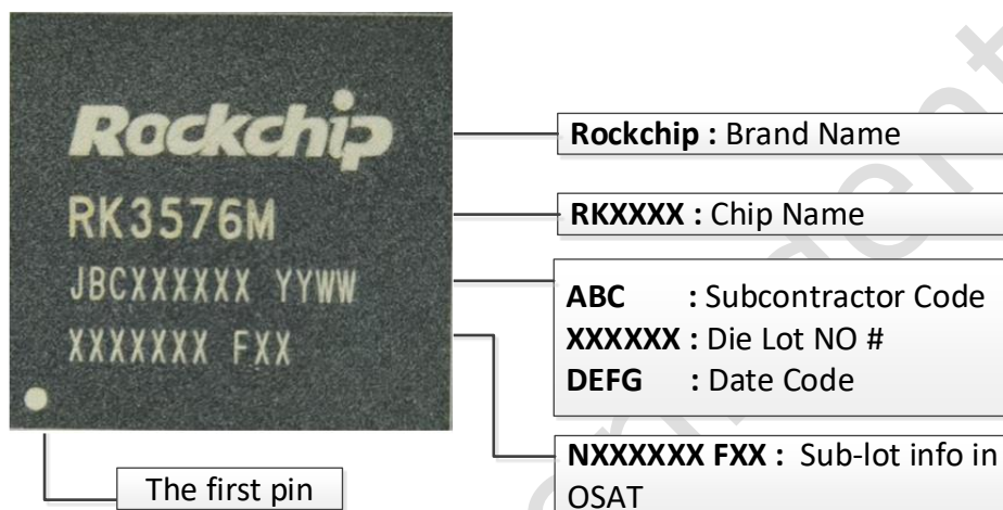
Fig.2-1 Package Definition
