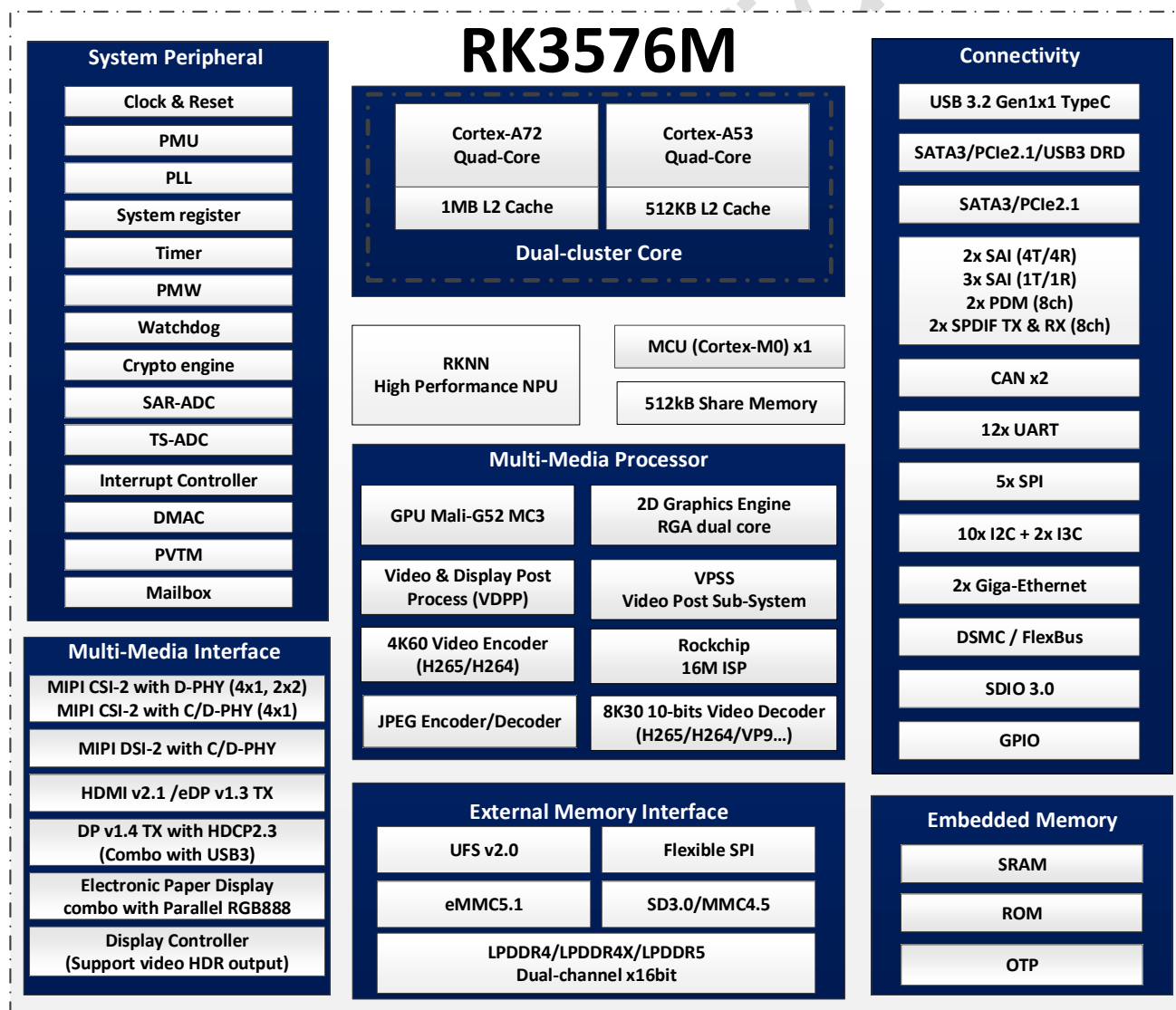
Fig.1-1 Block Diagram
