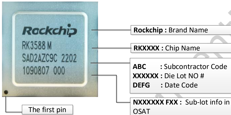
Fig.2-1 Package definition
