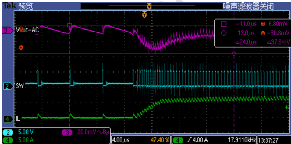
Fig. 4-6 BUCK1 load transient rising edge
