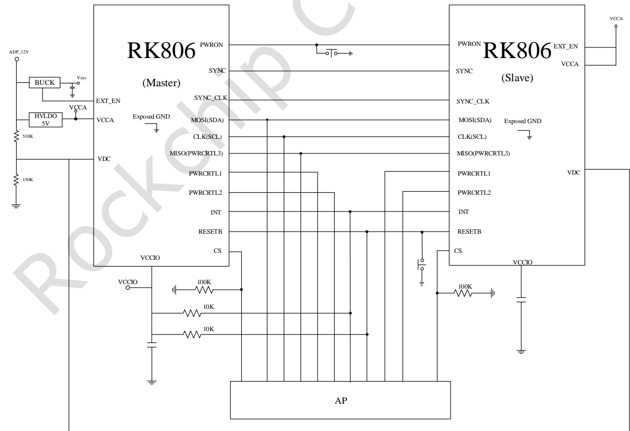
Fig. 1-4 Two RK806 Typical Application Diagram (SPI communication mode)
