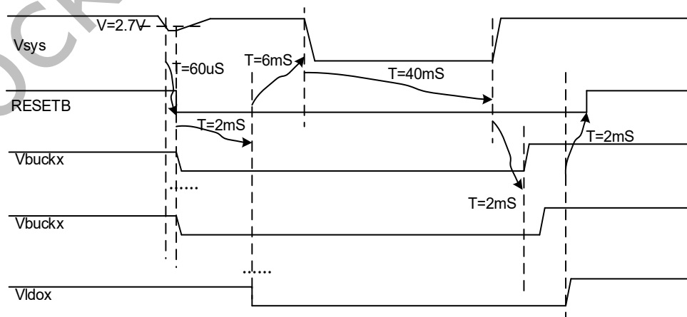
Fig. 4-7 VSYS under-voltage to restart the PMIC
