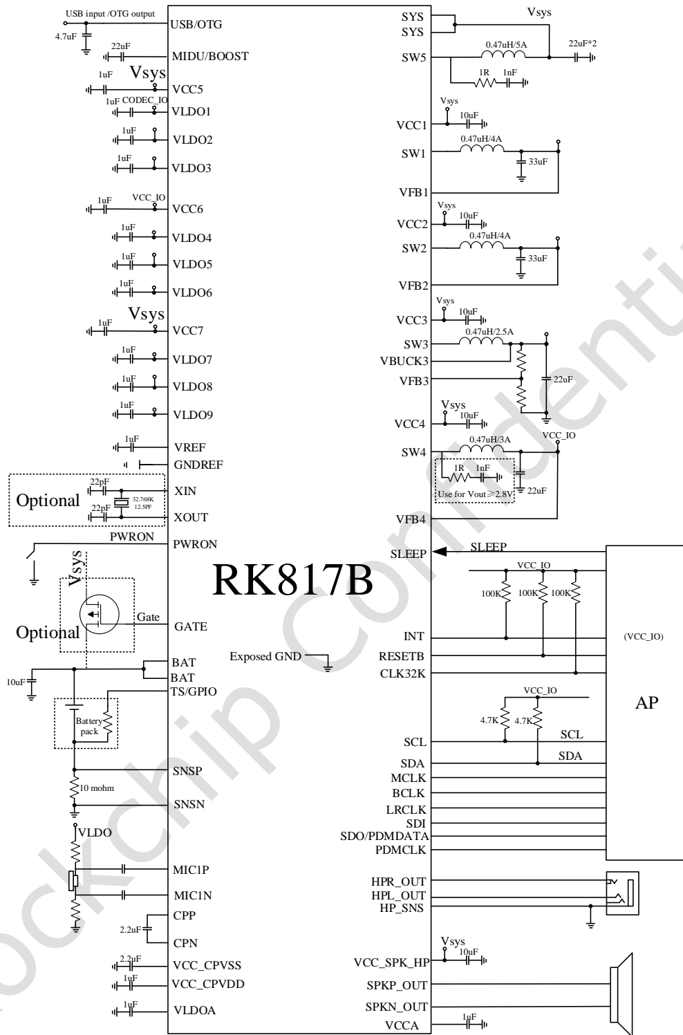
Fig. 1-2 RK817B Typical Application Diagram
