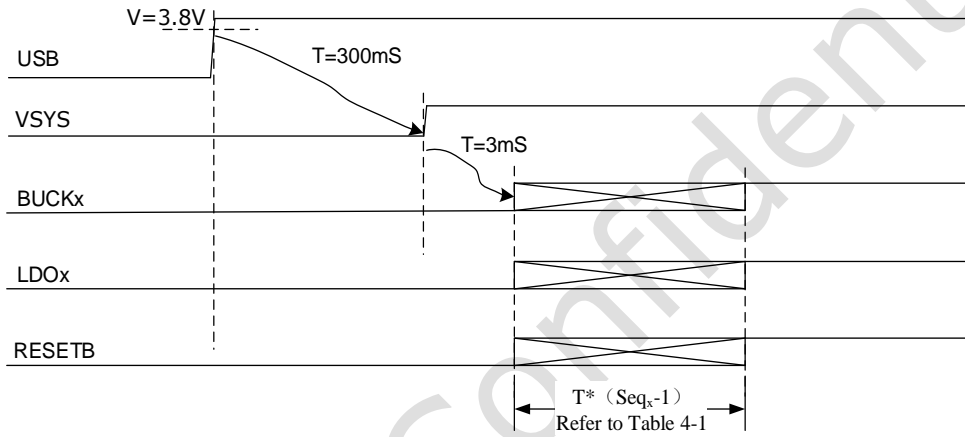
Fig. 4-3 USB plug in to turn on the PMIC without battery
