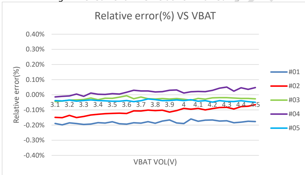
Fig. 4-20 Voltage ADC Relative Error Curve
