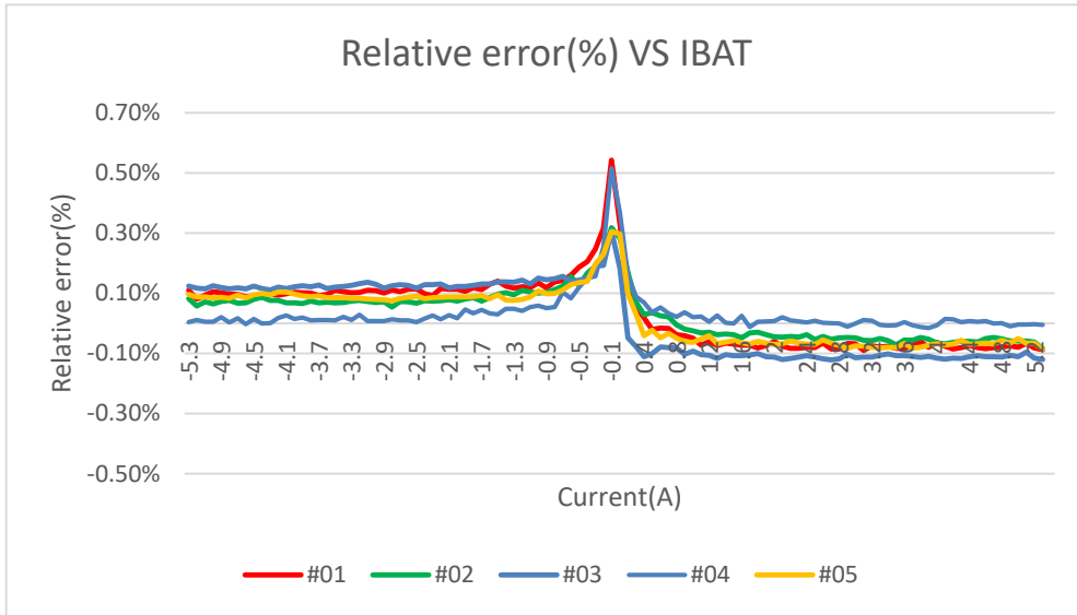
Fig. 4-19 Current ADC Relative Error Curve
