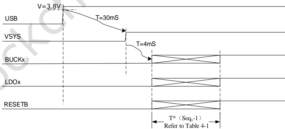
Fig. 4-4 USB plug in to turn on the PMIC with a battery
