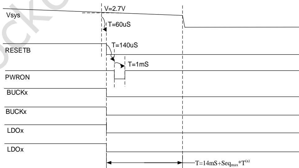
(a):Seqmax is maximum number of the shutdown sequence refer to Register 0x68~0x6E(7 bits I2C address is 0x22), T refer to Table 4-1 Sequence gap.
