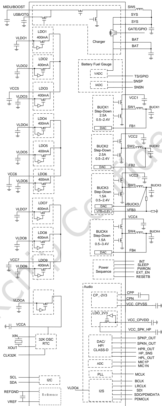
Fig. 1-1 RK817B Functional Block Diagram
