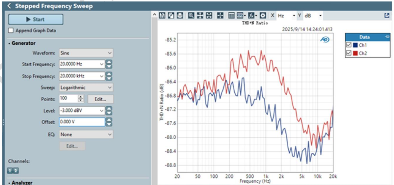
Fig. 4-22 Audio recording path THD+N ratio at differential mode
