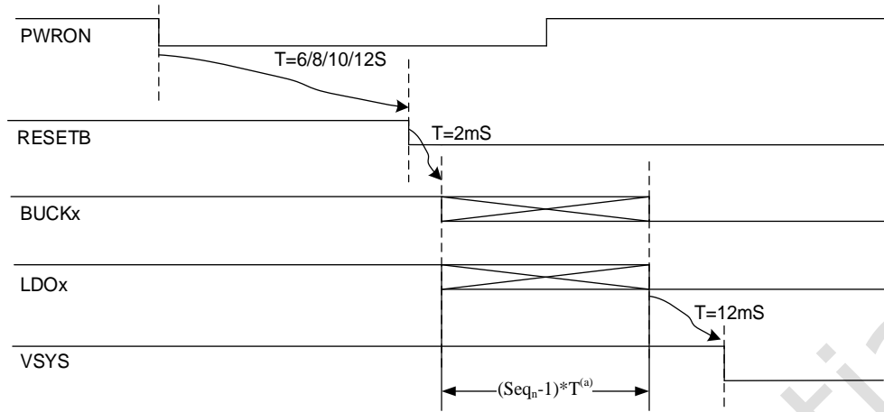
(a):Seqn is the number of shutdown sequence refer to Register 0x68~0x6F(7 bits I2C address is 0x22), T refer to Table 4-1 Sequence gap
