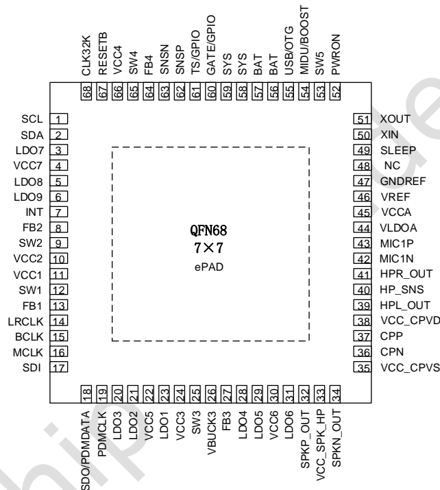
Fig. 2-2 Pin Assignment QFN7x7-68(Pitch=0.35mm)
