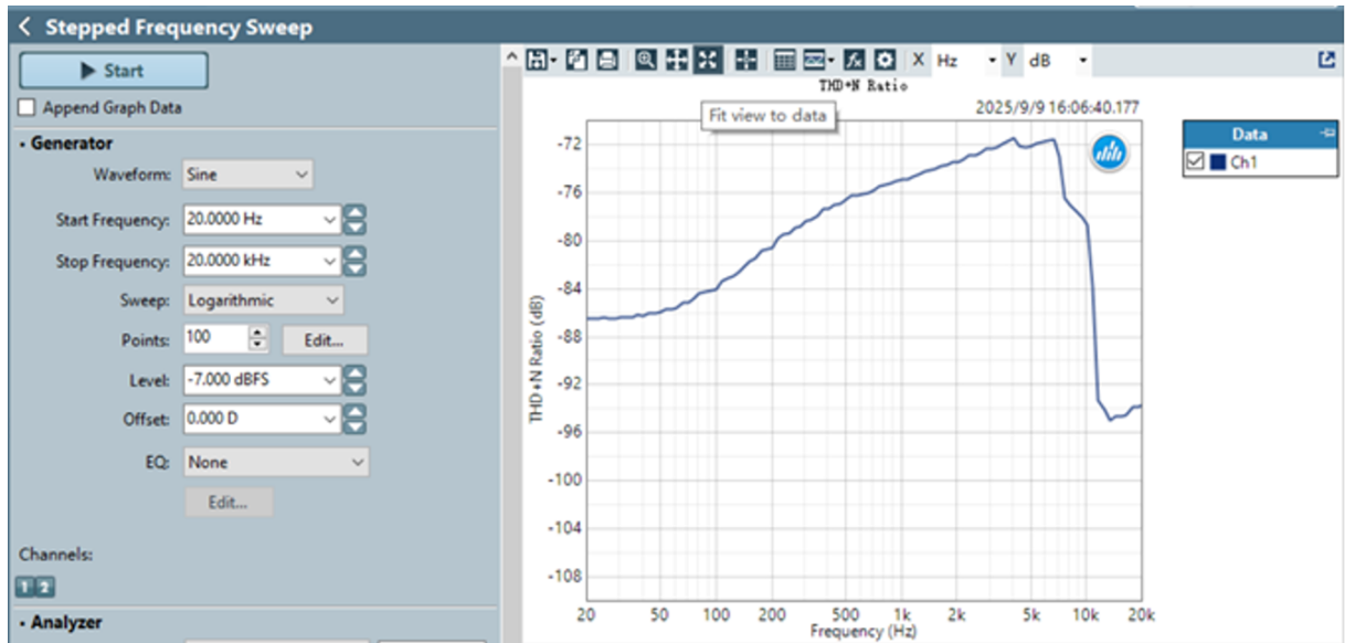
Fig. 4-24 Speaker path THD+N ratio
