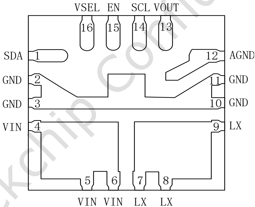
Fig. 1-3 Pin Assignment (Top view)
