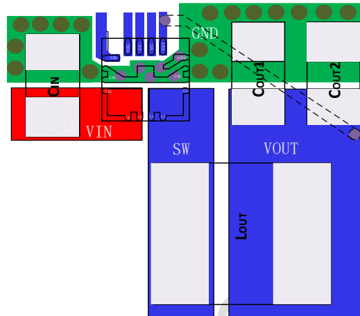
Fig. 6-2 PCB Layout Suggestion
