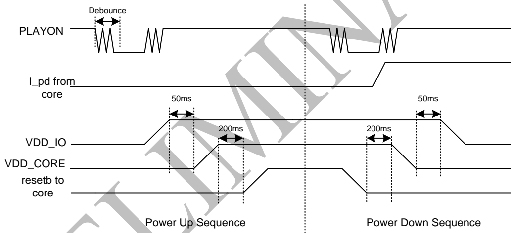
Fig. 7-3 Normal Power On/Off Sequence
