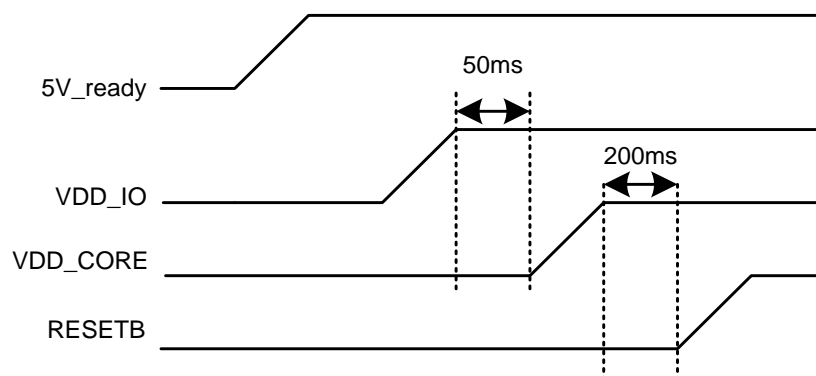
Fig. 7-4 Adapter Plug-In Power On Sequence
