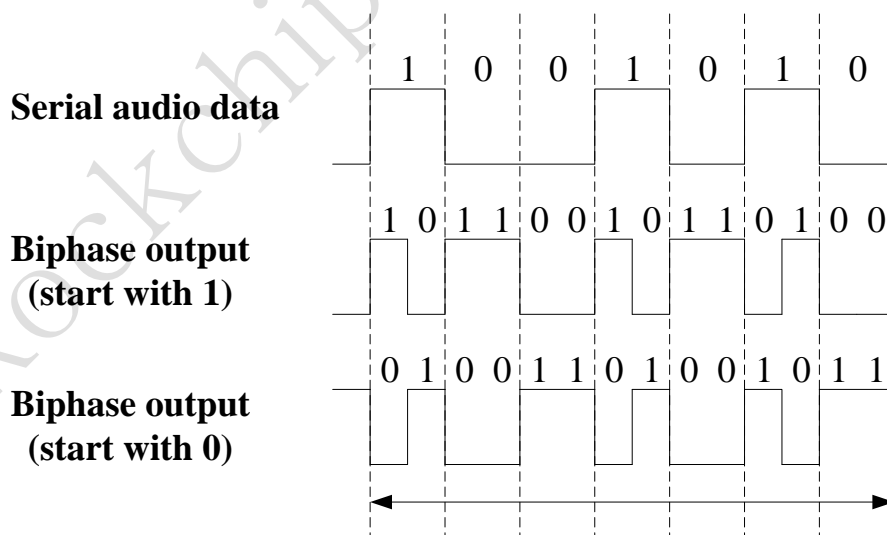
Fig. 30-4SPDIF Channel Coding
