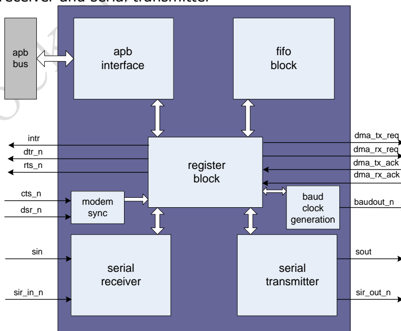
Fig. 36-1UART Architecture
