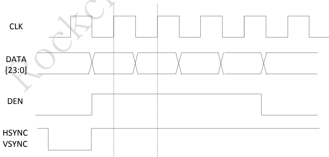
Fig. 22-19 LCDC RGB LCD interface (SDR mode)
