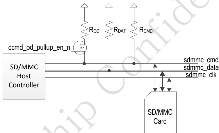
Fig. 17-7 SD/MMC Termination
