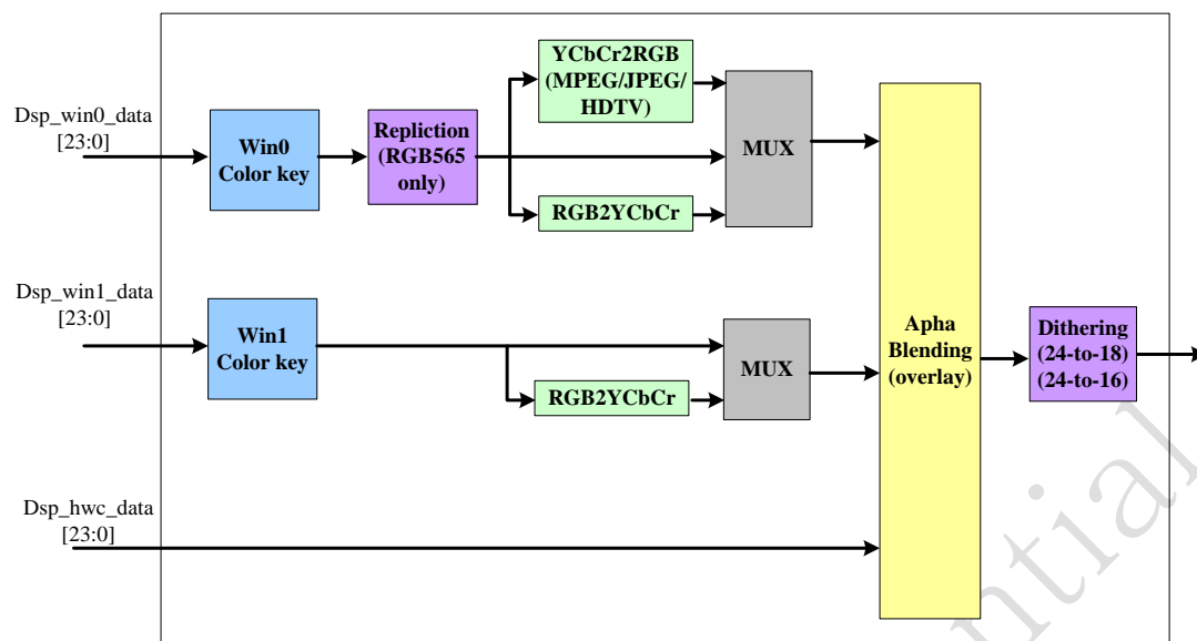
Fig. 22-12 LCD Overlay Block Diagram
