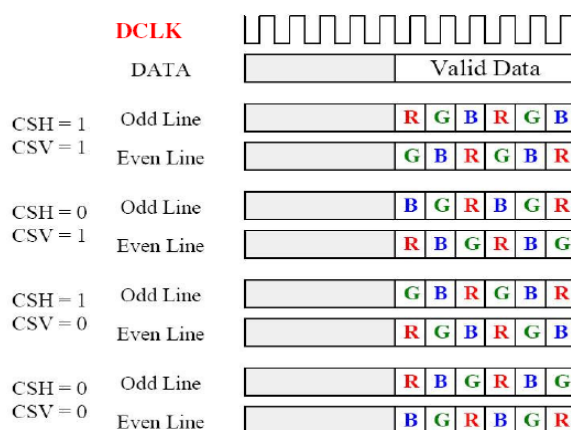
Fig. 22-22 LCDC RGB delta LCD interface
