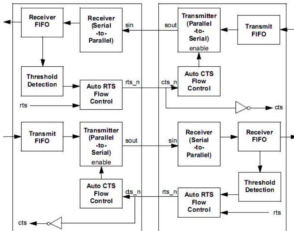
Fig. 36-4UART Auto flow control block diagram
