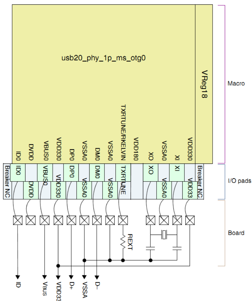
Fig. 1-9 RK3188 USB OTG/Host2.0 interface reference connection
