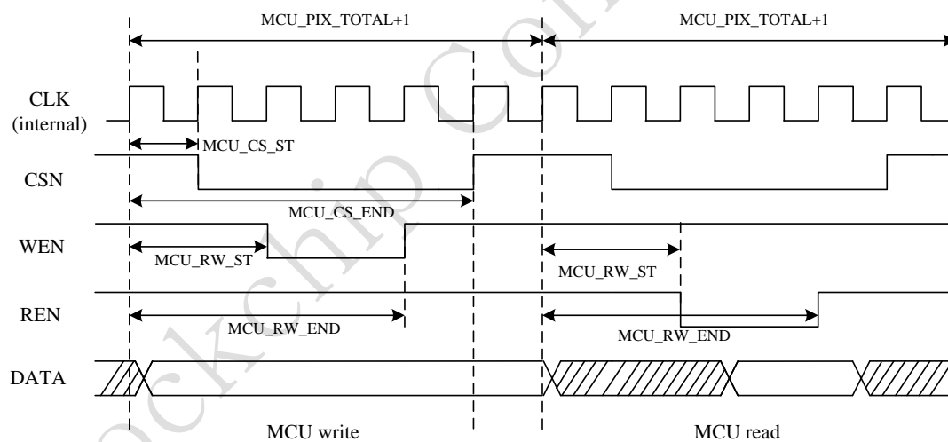
Fig. 22-21 LCDC MCU interface timing setting
