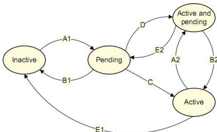
Fig. 12-2 GIC Interrupt handling state machine
