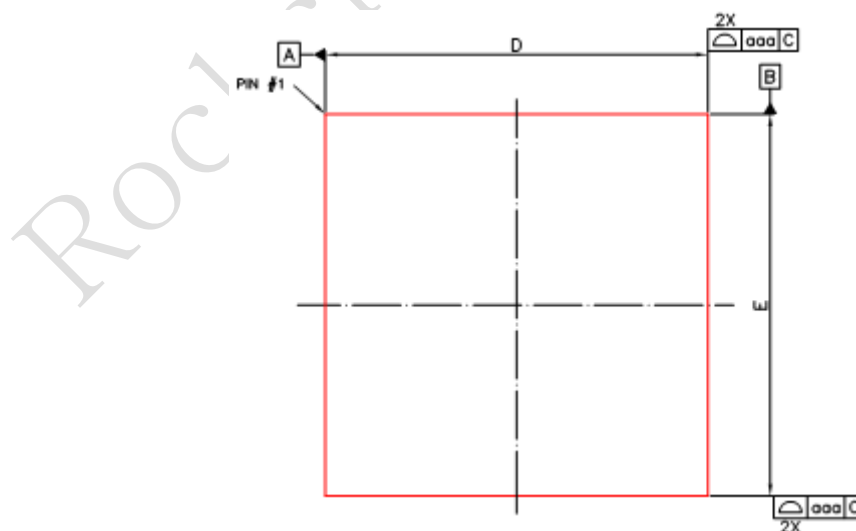
Fig. 1-2RK3188 TFBGA453 Package Top View
