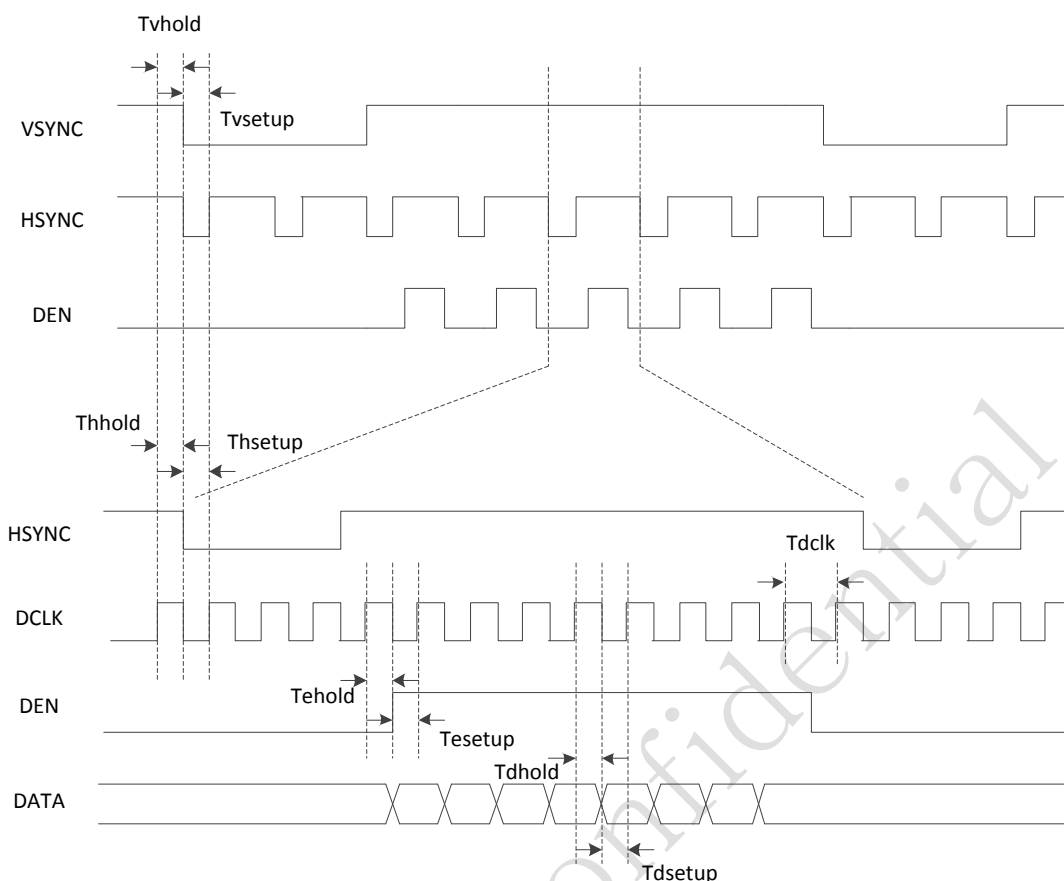
Fig. 22-23 LCD0 RGB interface timing (SDR)
