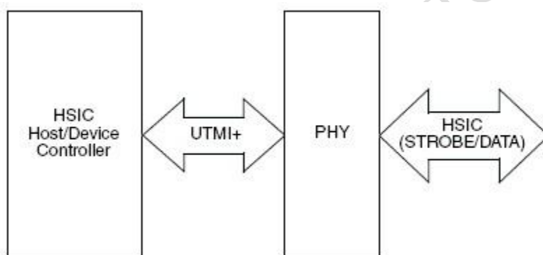
Fig. 27-1 USB HSIC Architecture
