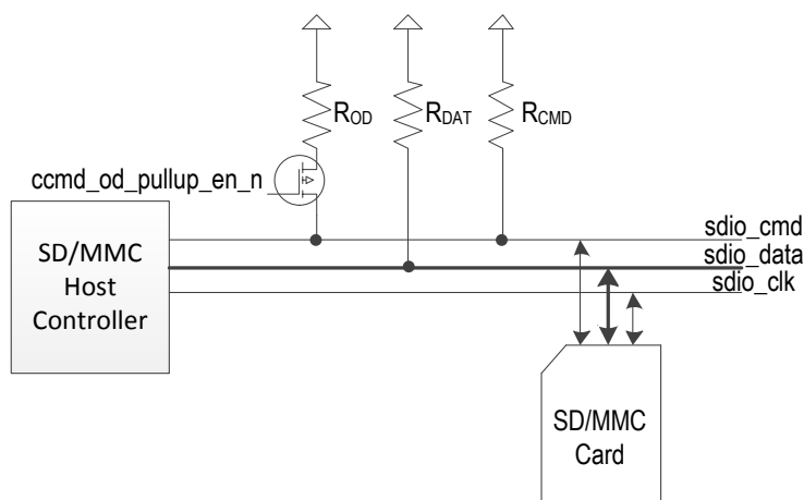
Fig. 31-3 SD/MMC Termination
