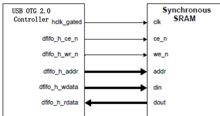
Fig. 26-11 DFIFO single-port synchronous SRAM interface
