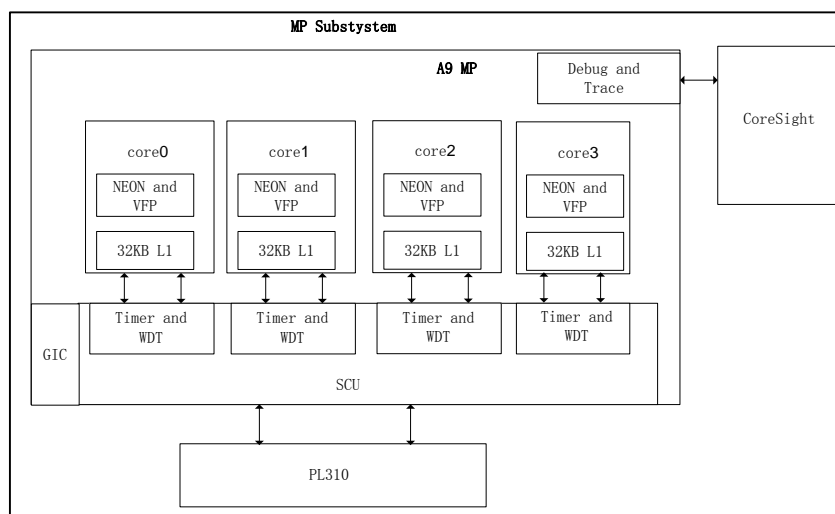
Fig. 8-1MP Subsystem architecture
