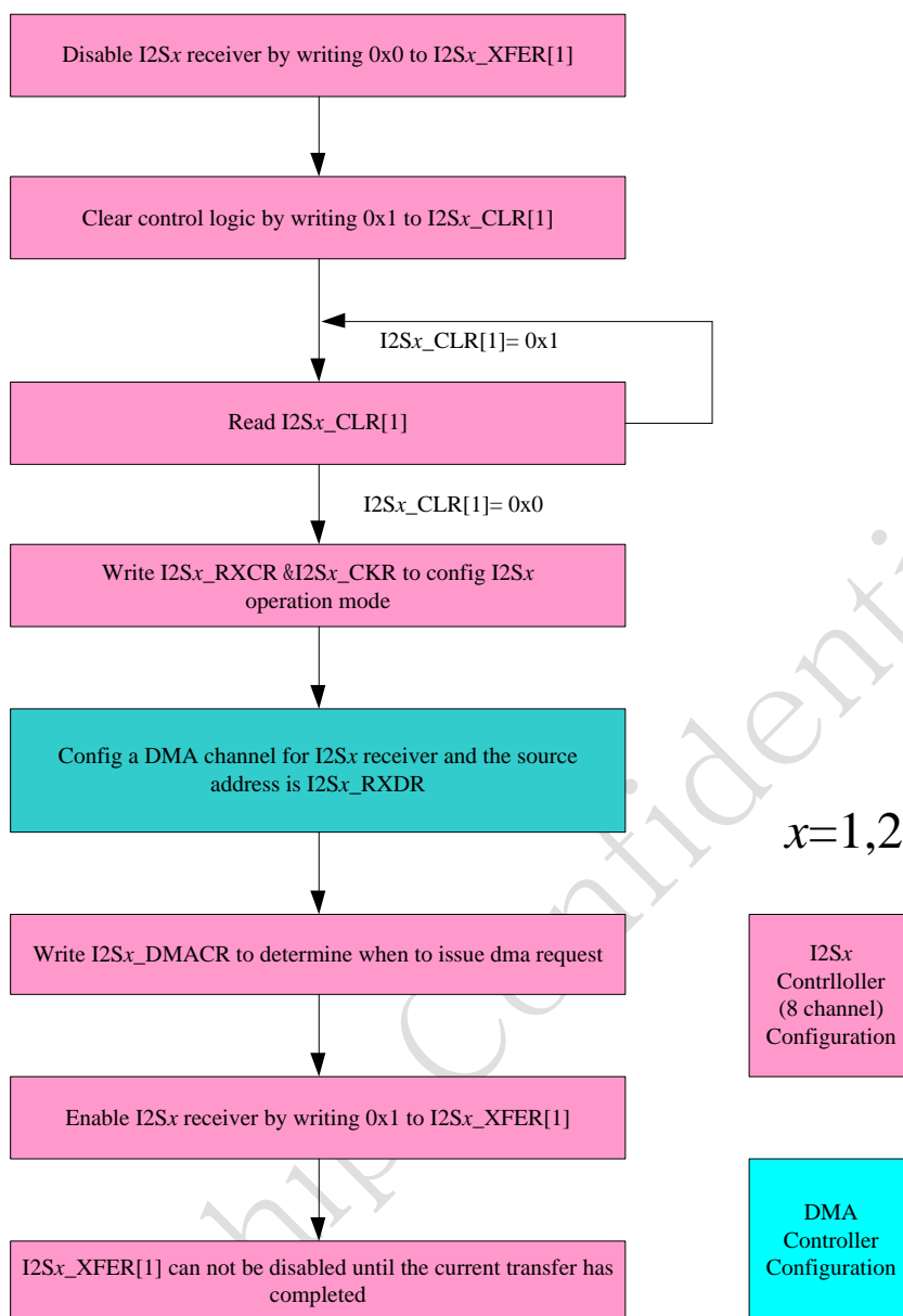
Fig. 29-14I2S/PCM1/2 controller receive operation flow chart
