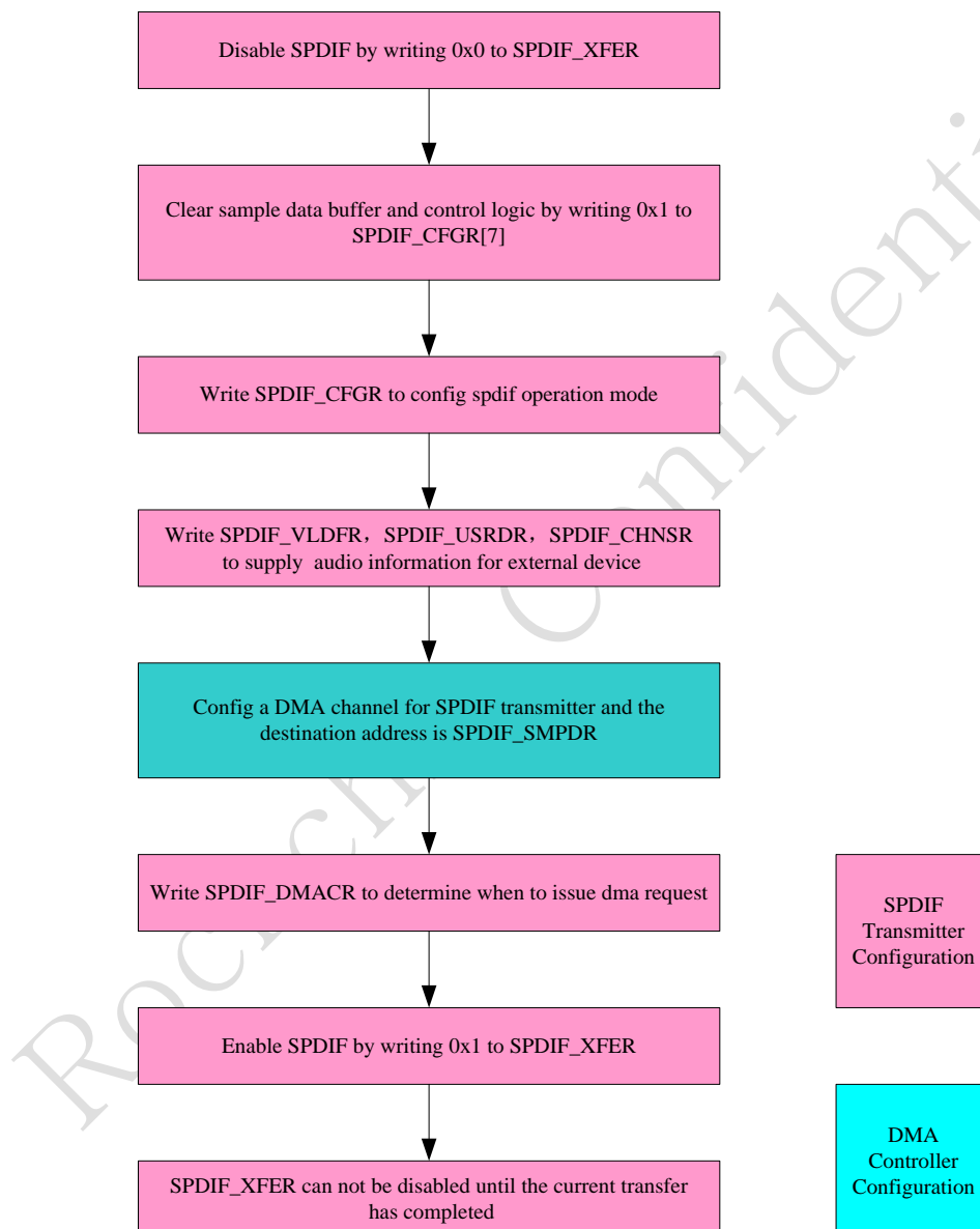
Fig. 30-6 SPDIF transmitter operation flow chart
