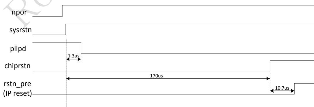
Fig. 1-10 RK3188 reset signals sequence
