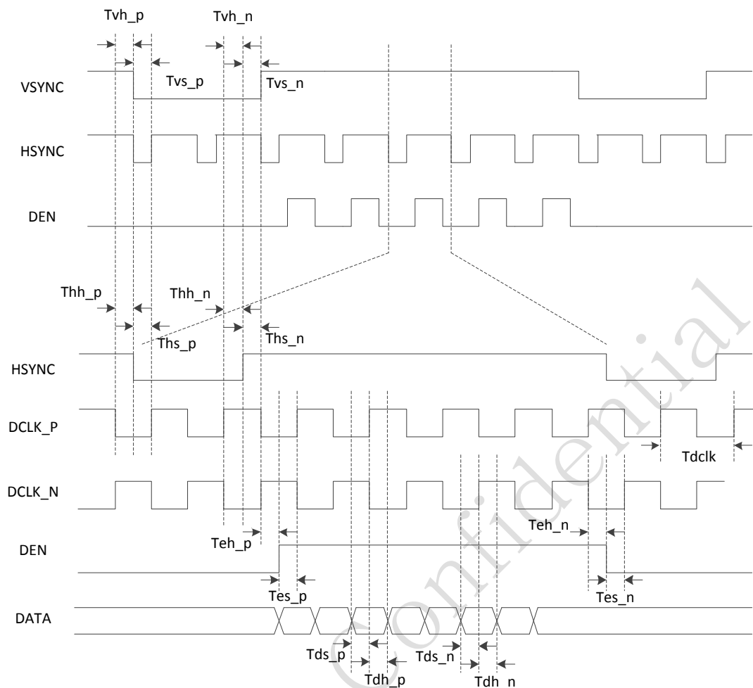
Fig. 22-24 LCDC RGB interface timing (DDR)
