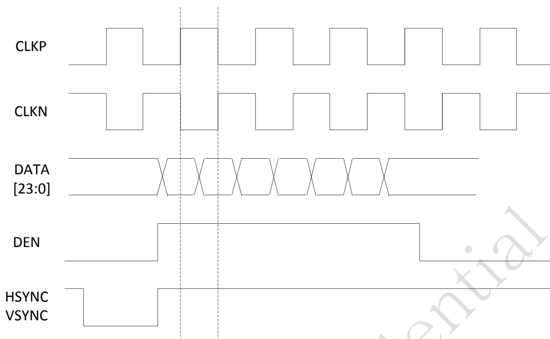
Fig. 22-20 LCDC RGB LCD interface (DDR mode)
