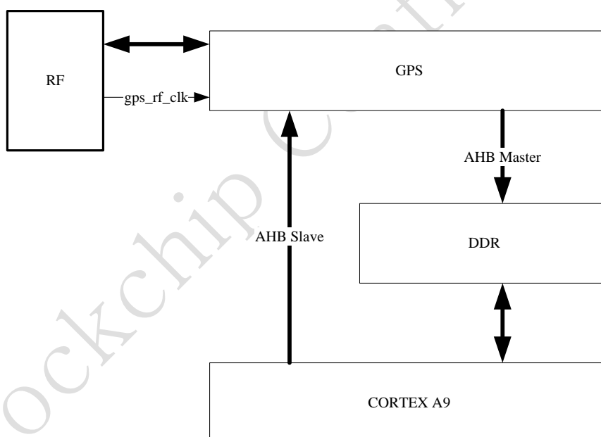
Fig. 28-1RK3188 GPS block diagram
