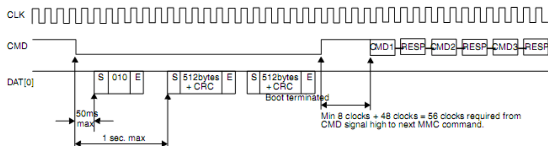
Fig. 17-10 Boot Operation
