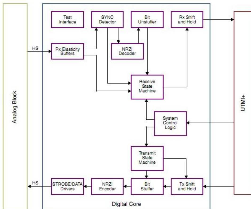
Fig. 27-4USB HSIC PHY Digital Block Architecture
