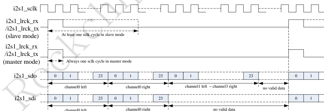
Fig. 29-7PCM early mode timing format
