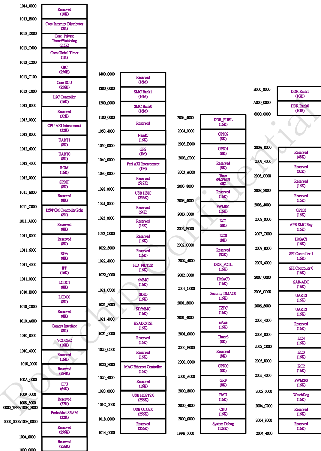
Fig. 2-2RK3188 Address Mapping after remap
