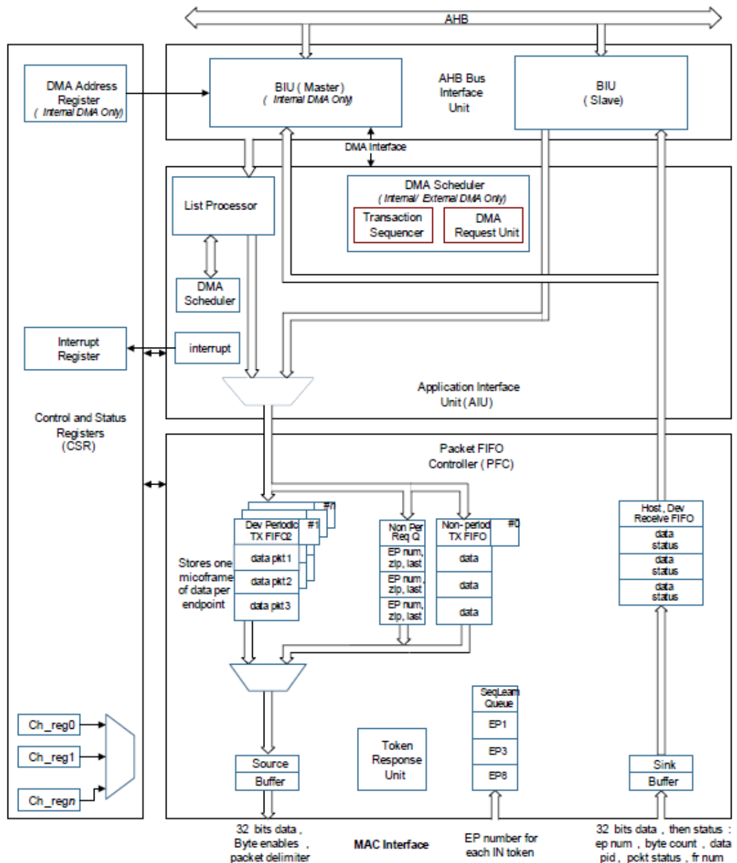
Fig. 26-6 USB OTG2.0 Controller – Host Architecture
