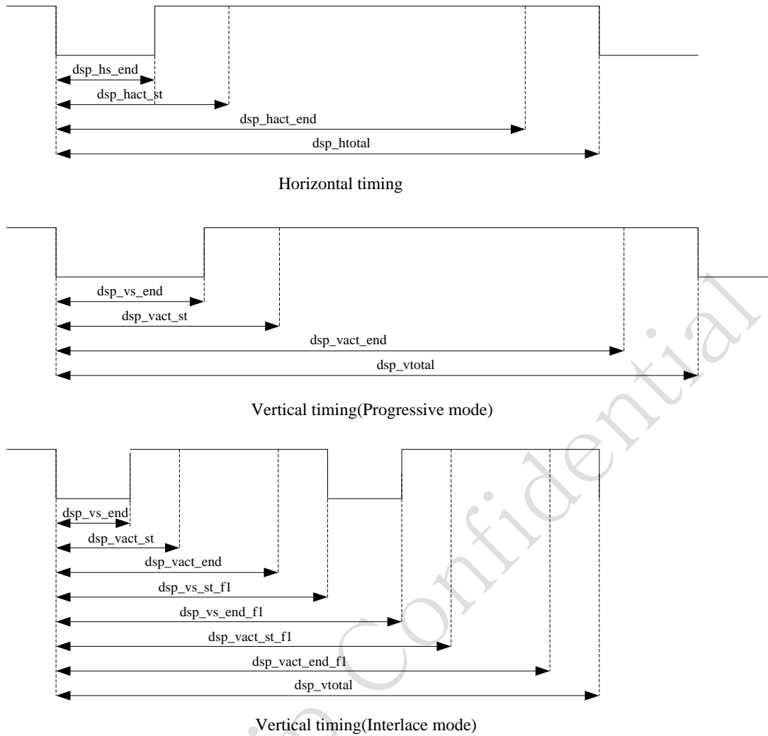
Fig. 22-18 LCDC RGB interface timing setting
