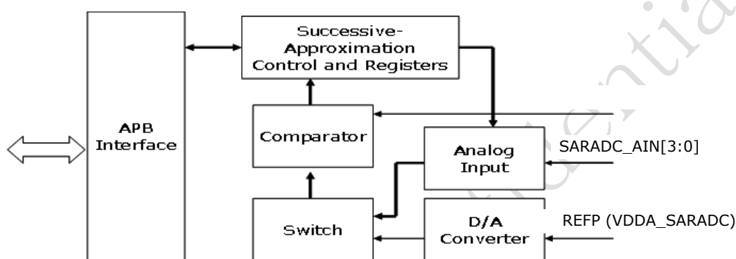
Fig. 42-1RK3188 SAR-ADC block diagram
