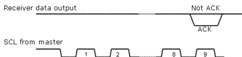
Fig. 37-4I2C Acknowledge
