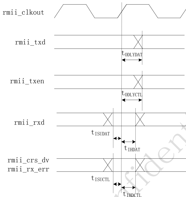
Fig. 32-6 RMII timing diagram
