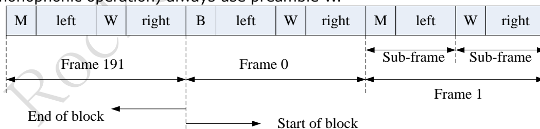
Fig. 30-2SPDIF Frame Format
