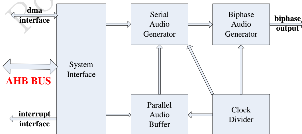
Fig. 30-1SPDIF transmitter Block Diagram
