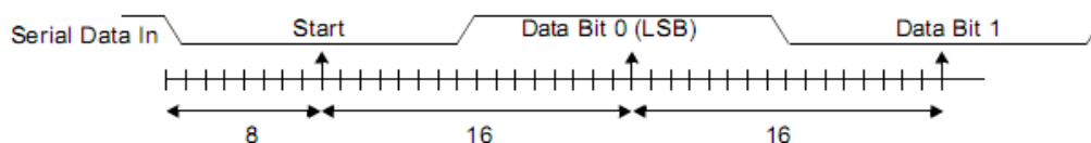
Fig. 36-3UART baud rate
