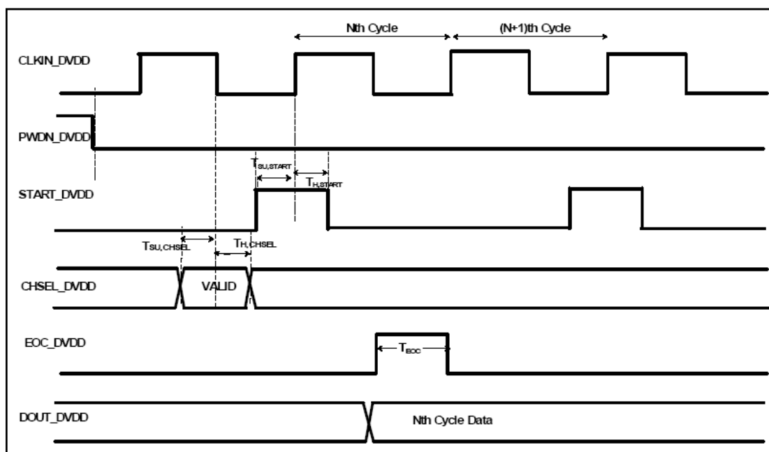
Fig. 42-2SAR-ADC timing diagram in single-sample conversion mode
