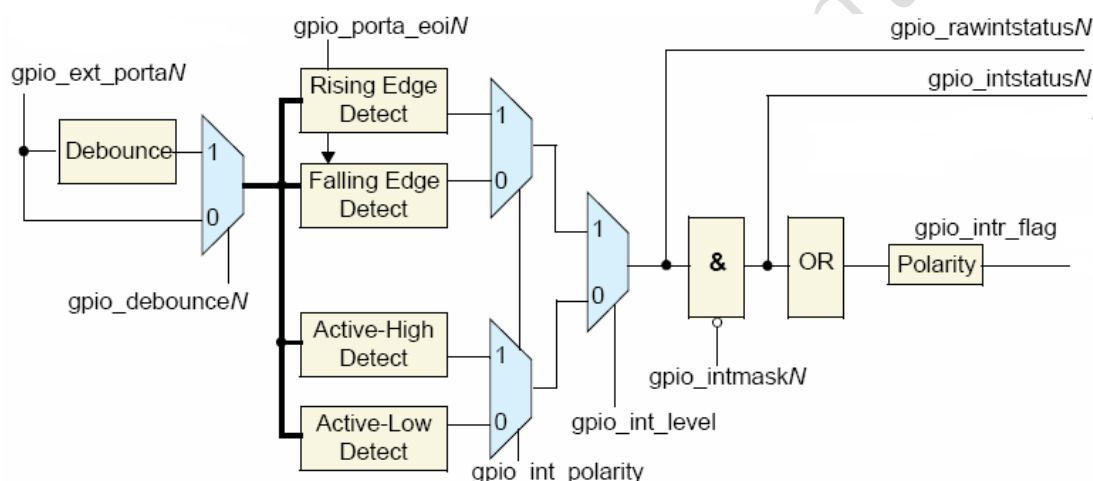
Fig. 38-2 Interrupt RTL Block Diagram
