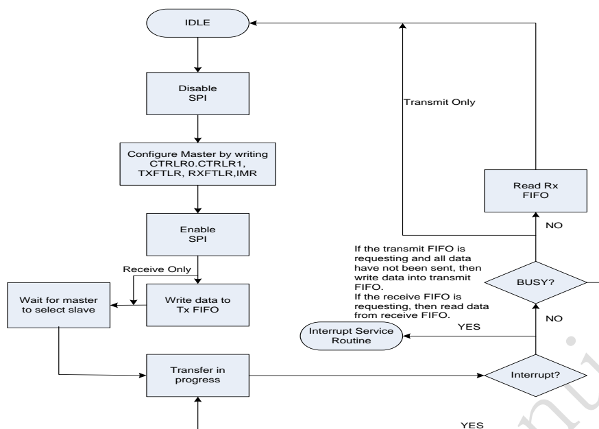
Fig. 35-10SPI Slave transfer flow diagram
