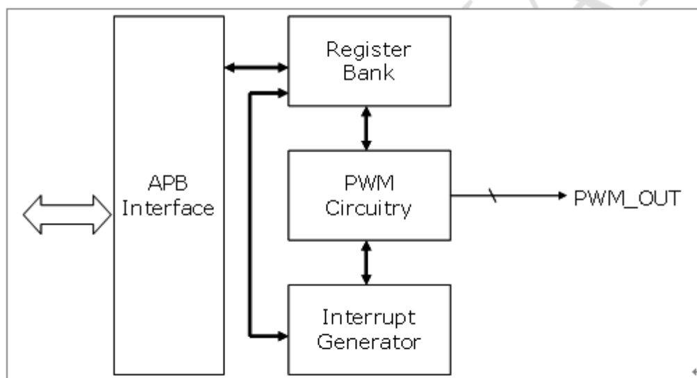
Fig. 40-1 PWM architecture
