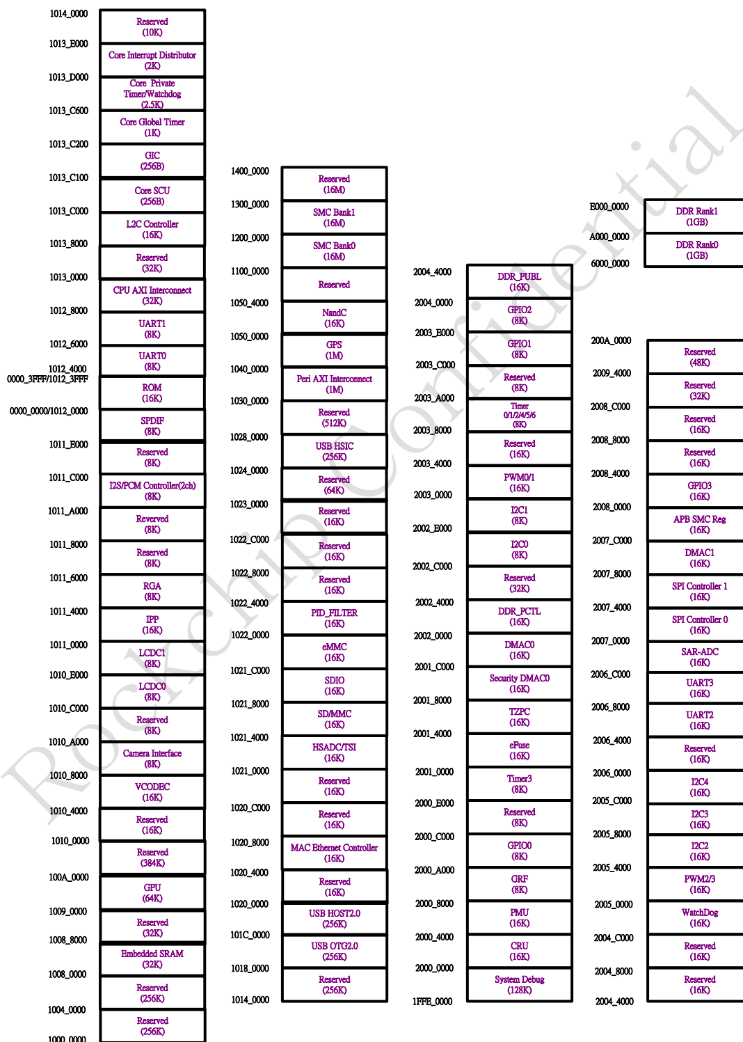
Fig. 2-1RK3188 Address Mapping before remap
