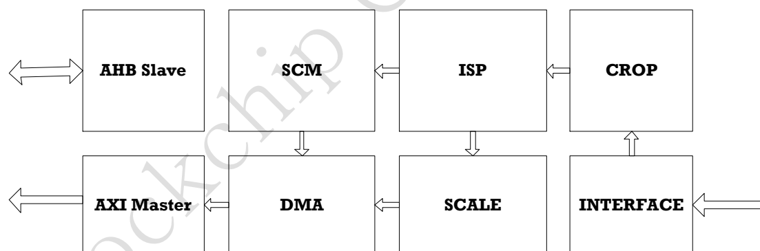
Fig. 24-1CIF block diagram
