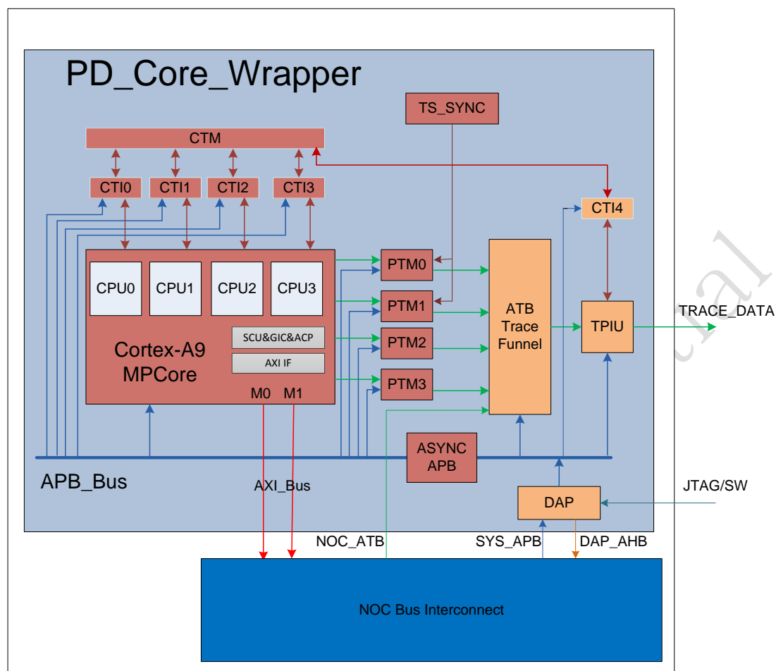
Fig. 6-1RK3188 Debug system structure
