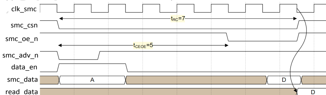
Fig. 14-4 SMC asynchronous read timing in multiplexed mode
