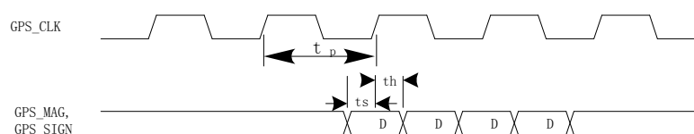
Fig. 28-2RK3188 GPS timing waveform
