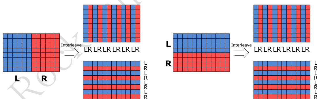
Fig. 22-11LCD Interleave 3D Display
