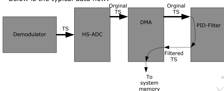
Fig. 34-2 PID-Filter data flow
