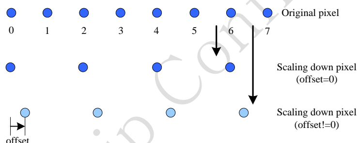
Fig. 22-7LCDC Scaling Down Offset
