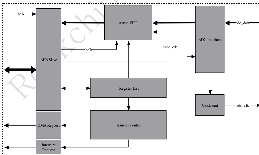
Fig. 33-1 HS-ADC/TS Interface block diagram
