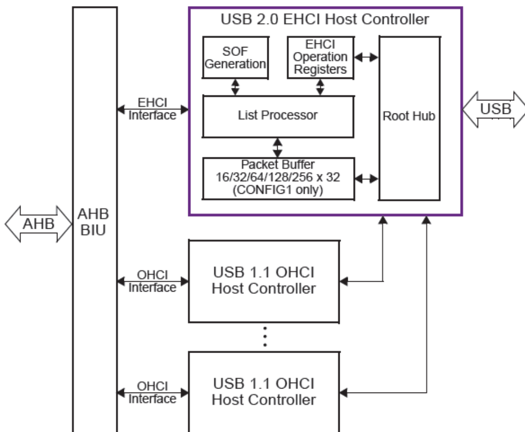
Fig. 27-2 USB HSIC Controller Architecture
