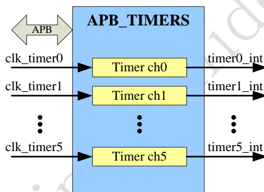
Fig. 39-1 TimersBlock Diagram
