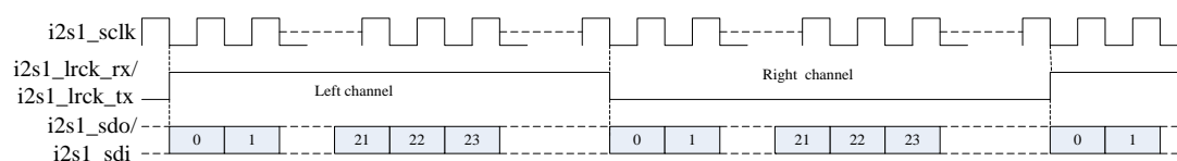
Fig. 29-5I2S left justified mode timing format
