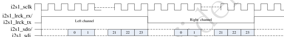
Fig. 29-6I2S right justified mode timing format
