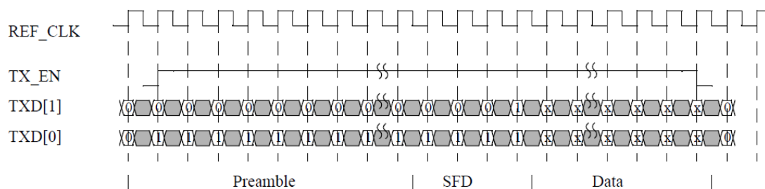
Fig. 32-3RMII transmission in 100Mb/s mode
