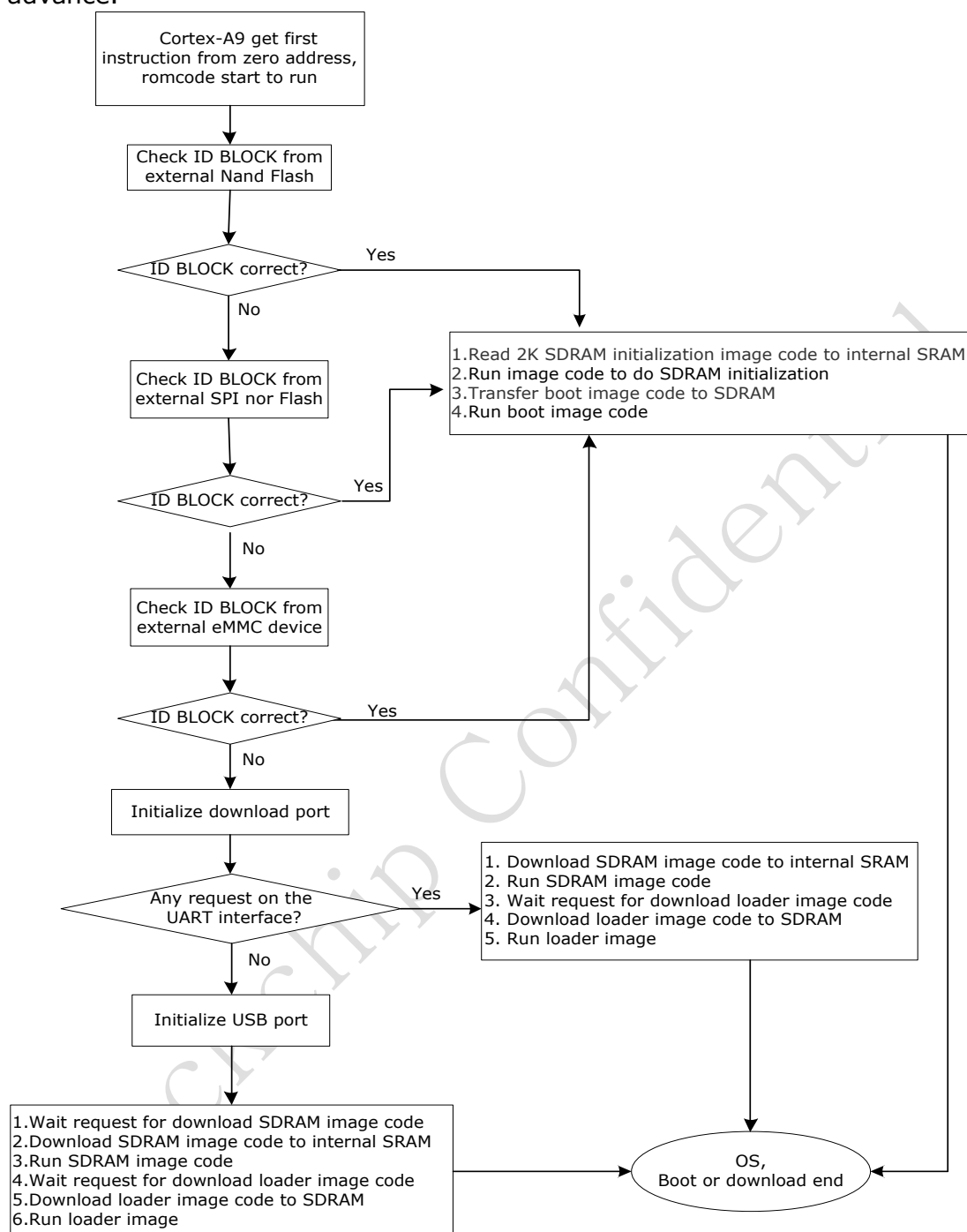
Fig. 2-3 RK3188 boot procedure flow
