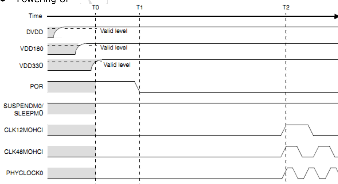
Fig. 26-14 USB OTG 2.0 PHY power supply and power up sequence
