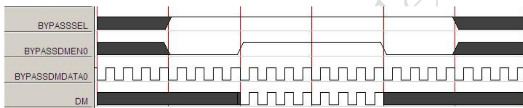
Fig. 26-16UART Timing Sequence
