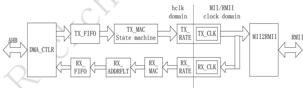
Fig. 32-1 VMAC architecture
