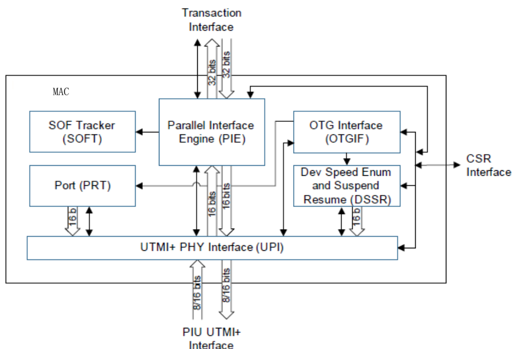
Fig. 26-12 USB OTG 2.0 Controller – MAC block diagram
