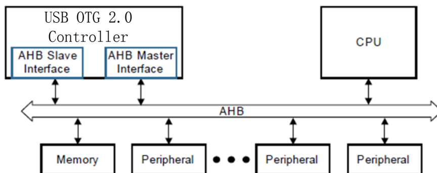
Fig. 26-7 USB OTG2.0 Controller – Internal DMA mode
