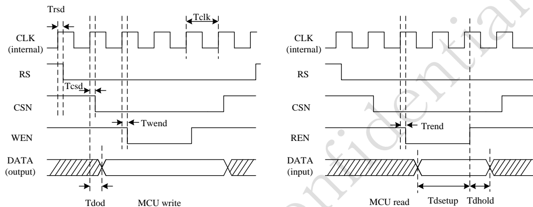
Fig. 22-25 LCDC MCU interface (i80)timing
