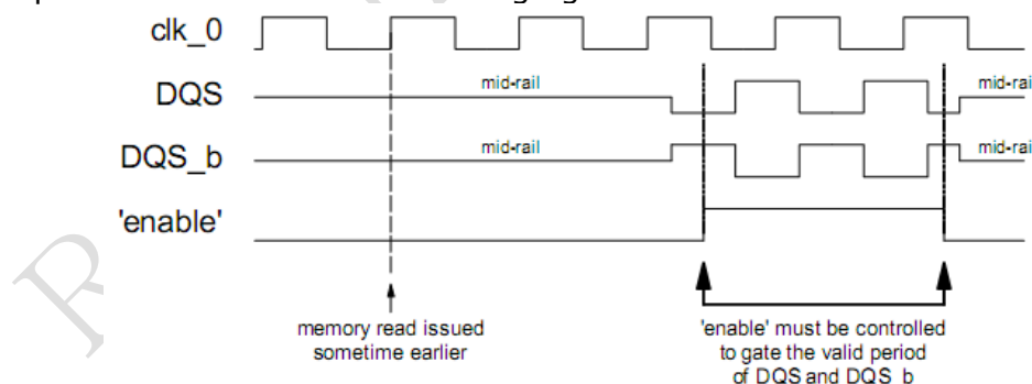
Fig. 13-7 Strobe Gating Requirements During Read Operations
