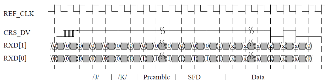
Fig. 32-4 RMII reception with no errors in 100Mb/s mode
