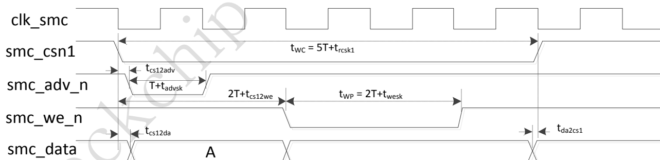
Fig. 14-10 Asynchronous Write Timing Diagram In Multiplexed Mode
