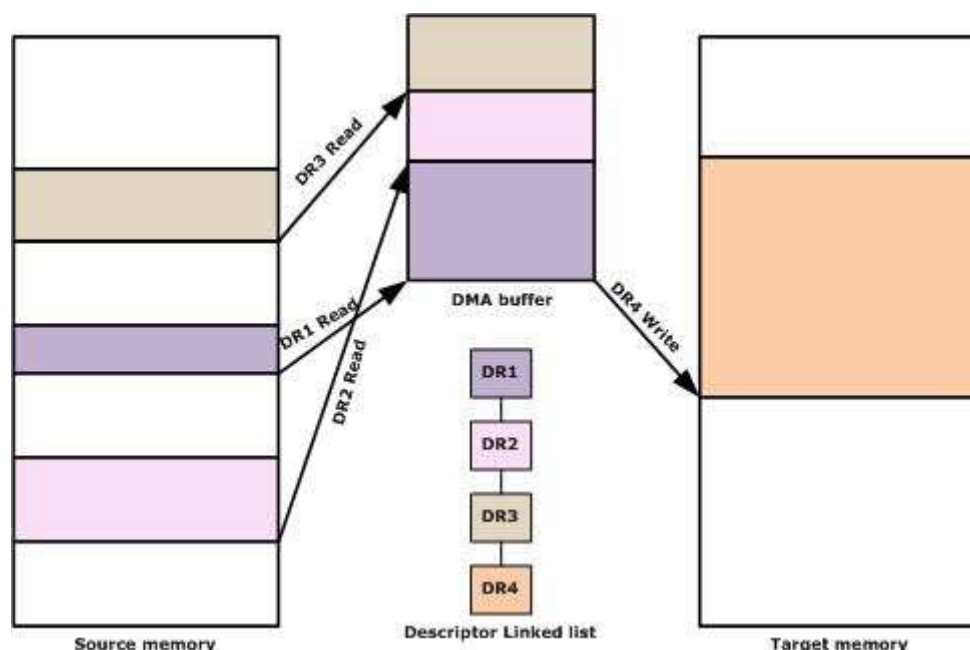
Fig. 17-22 Gathering data
