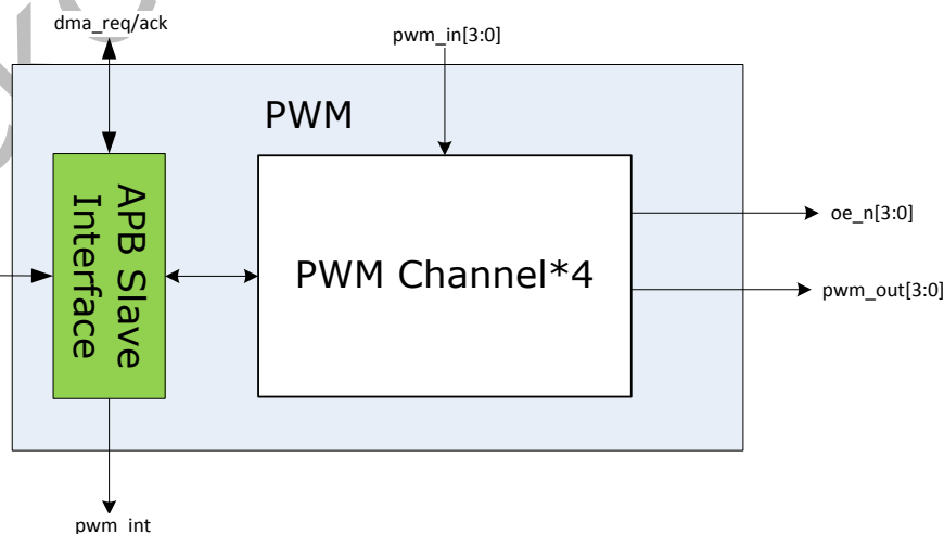
Fig. 8-1 PWM Block Diagram
