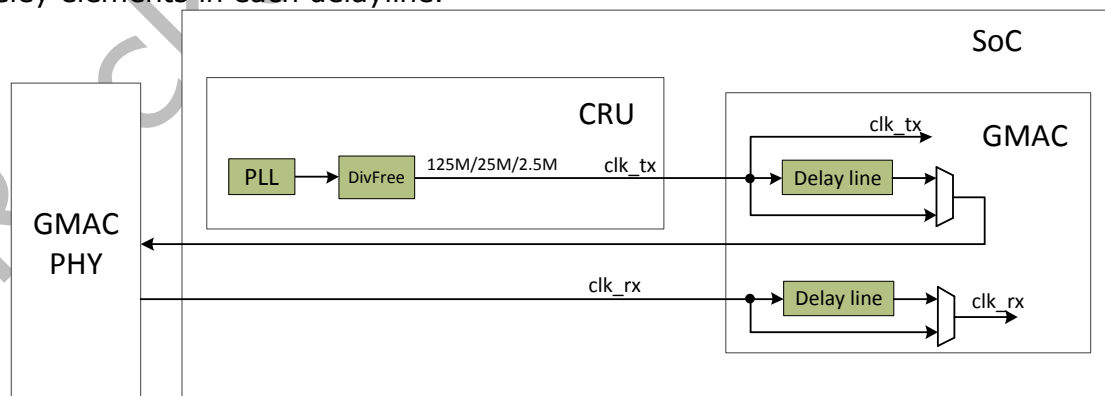
Fig. 15-14 RGMII clock architecture when clock source from CRU
