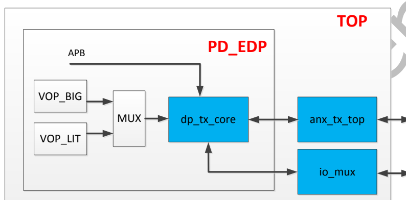
Fig. 6-2 edp TX controller in SoC
