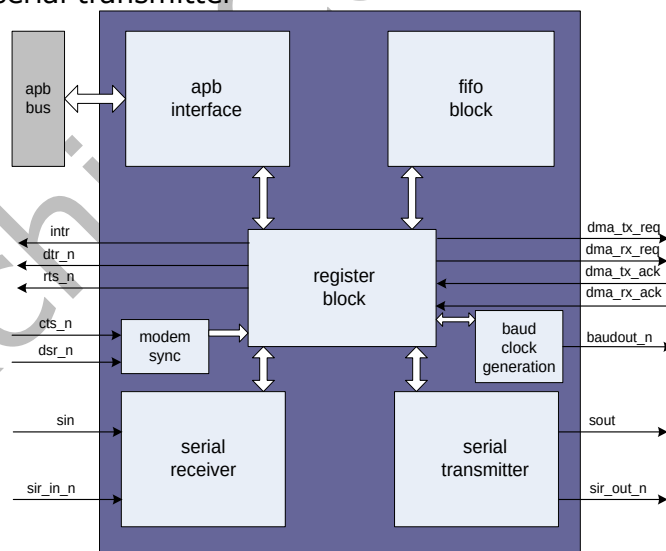
Fig. 9-1 UART Architecture
