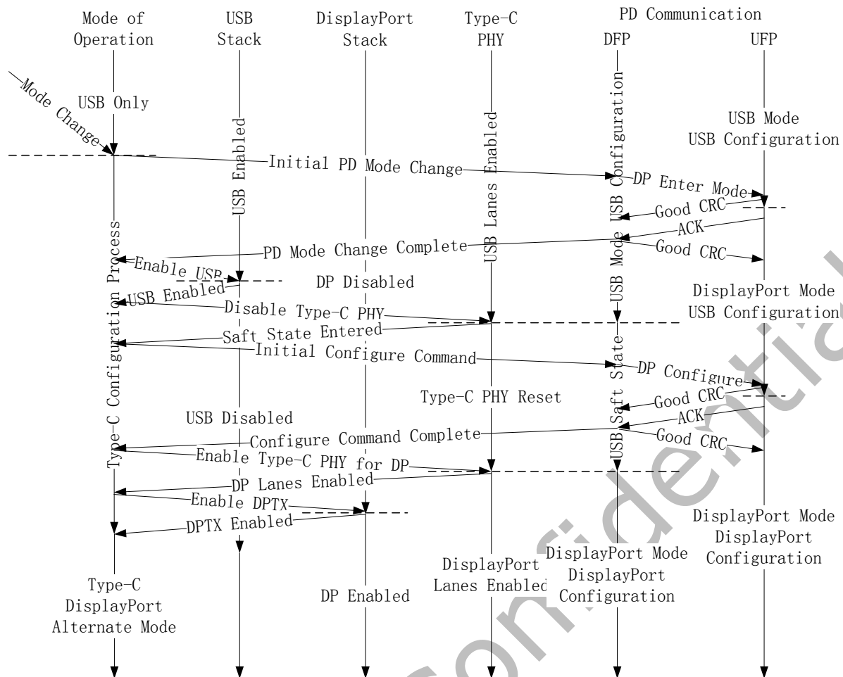
Fig. 18-5 Type-C Configuration Process
