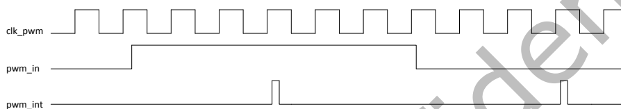
Fig. 8-2 PWM Capture Mode
