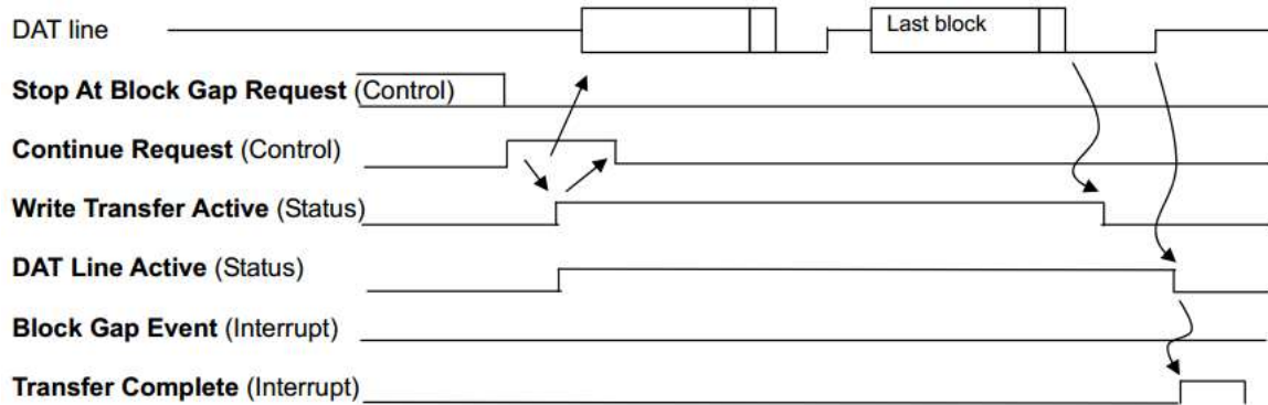
Fig. 16-24 Continue Write Transfer by Continue Request
