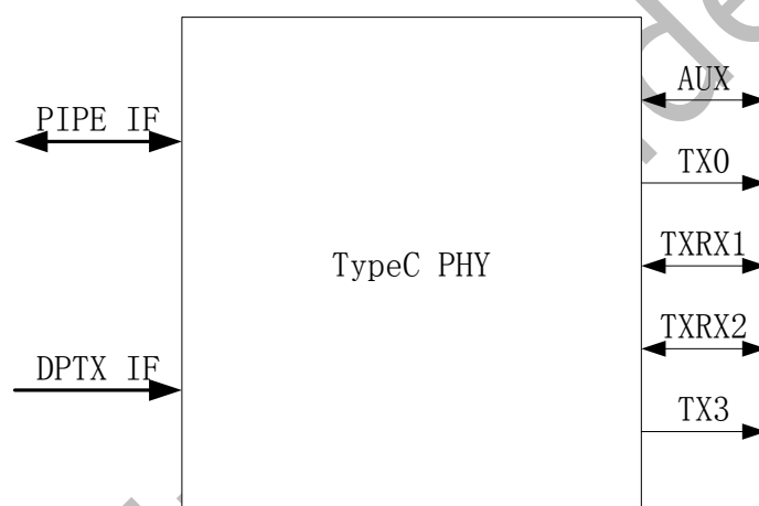
Fig. 19-1 TypC PHY Block Diagram
