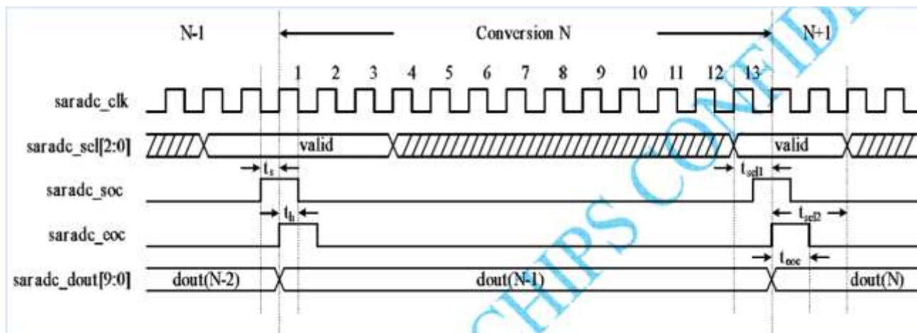
Fig. 20-2 SAR-ADC timing diagram in single-sample conversion mode
