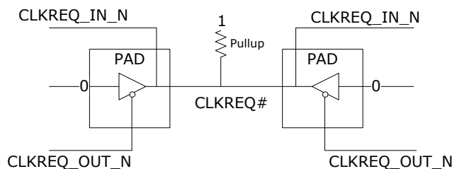
Fig. 17-29 Block Diagram of CLKREQ#
