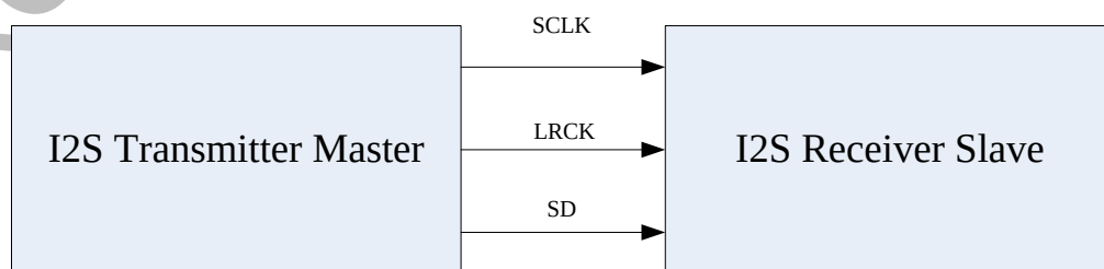
Fig. 12-2 I2S transmitter-master & receiver-slave condition
