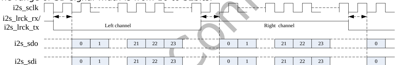
Fig. 12-4 I2S normal mode timing format
