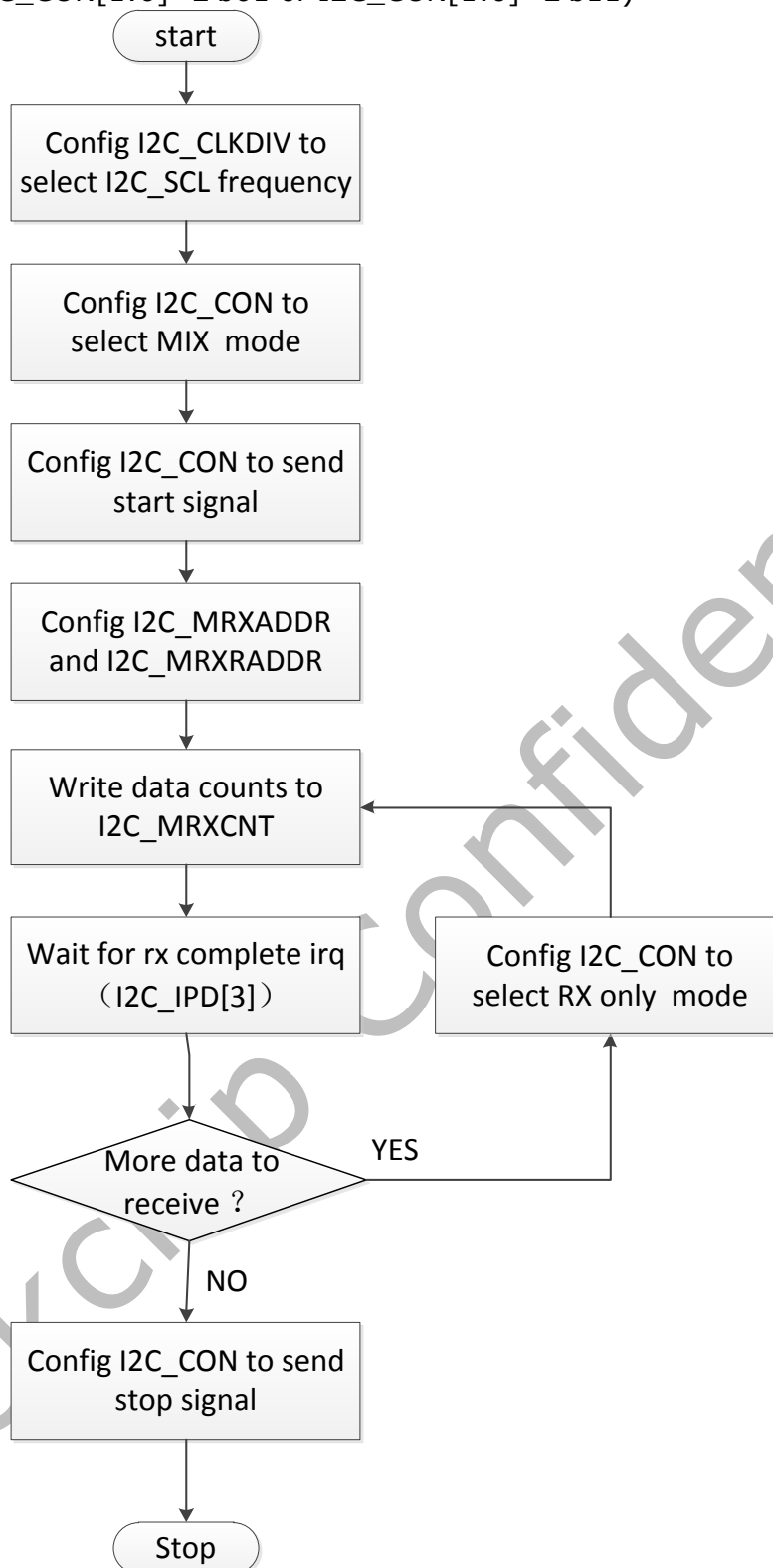
Fig. 11-8 I2C Flow chat for mix mode
