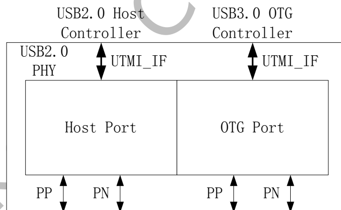
Fig. 2-1 USB2.0 PHY Block Diagram
