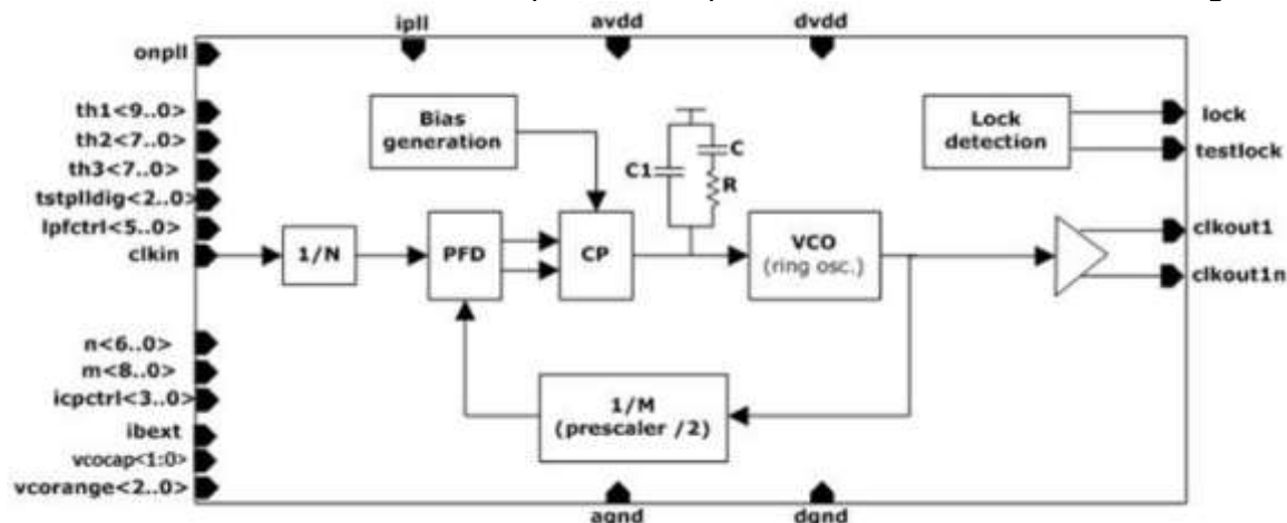
Fig. 7-5 PLL System-Level Block Diagram
