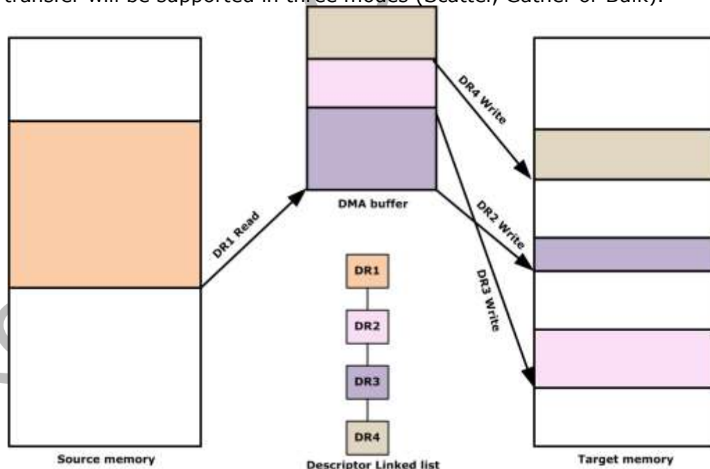
Fig. 17-21 Scattering data
