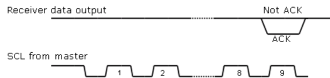
Fig. 11-4 I2C Acknowledge
