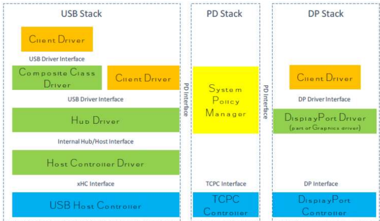
Fig. 18-2 TypeC Subsystem SW Architecture
