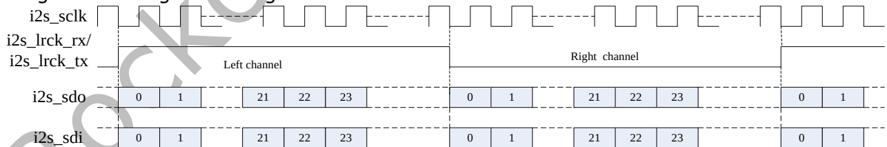
Fig. 12-5 I2S left justified mode timing format
