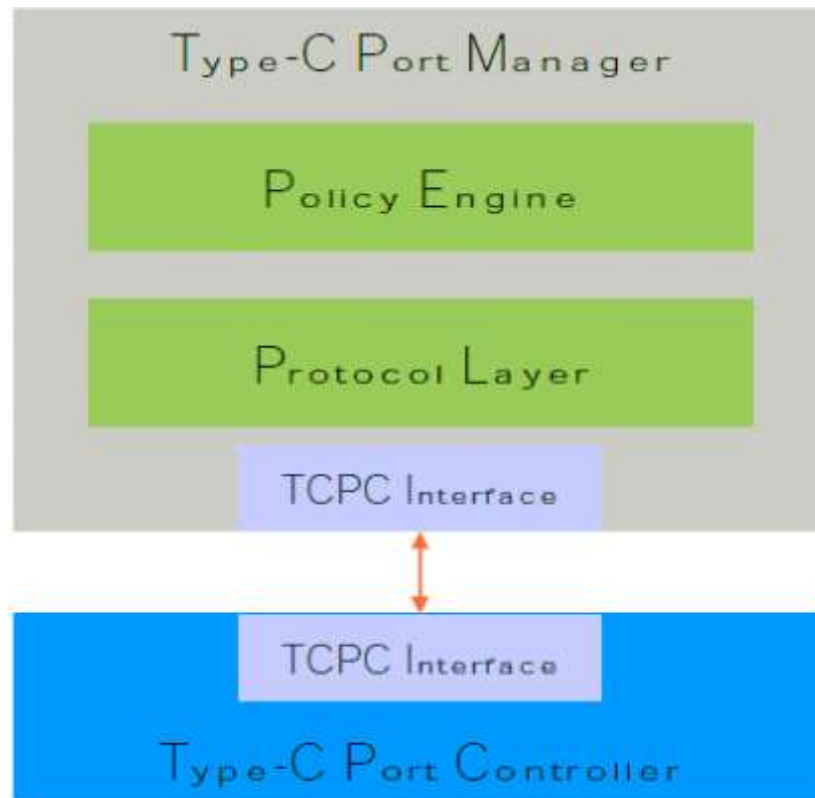
Fig. 18-3 Power Delivery SW Stack Architecture
