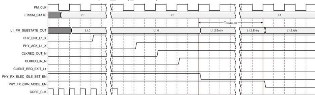
Fig. 17-34 L1.2 Substate Entry Operation
