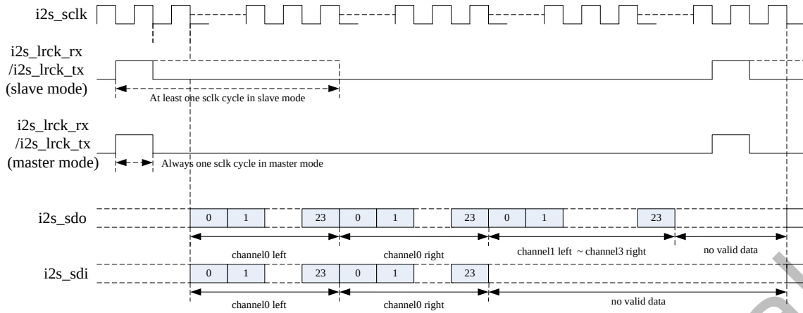
Fig. 12-9 PCM late2 mode timing format
