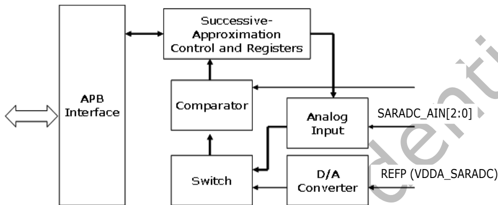
Fig. 20-1 RK3399SAR-ADC block diagram
