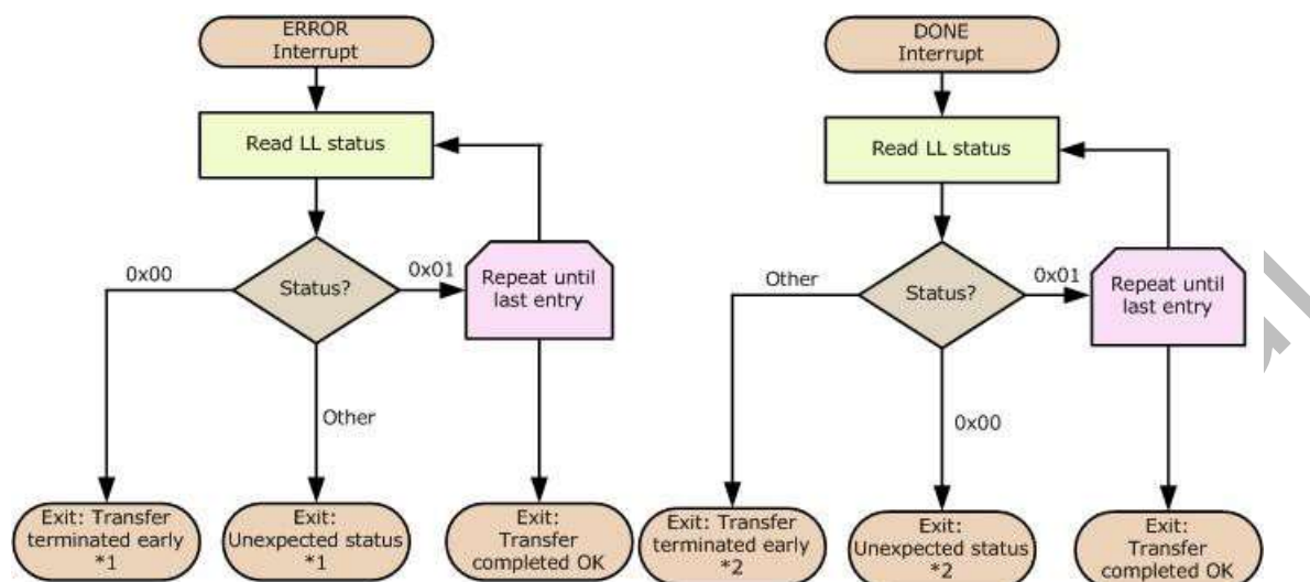
Fig. 17-26 Analysis of Transfer Complete
