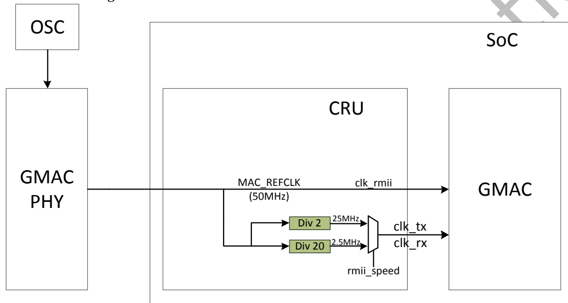
Fig. 15-13 RMII clock architecture when clock source from external OSC
