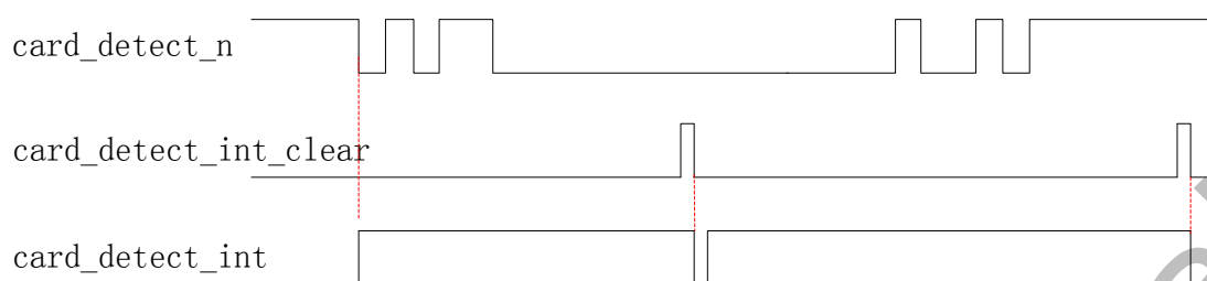
Fig. 1-20 Card Detection Method 4
