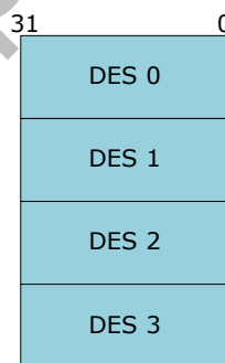
Fig. 1-8 Descriptor Formats for 32-bit AHB Address Bus Width
