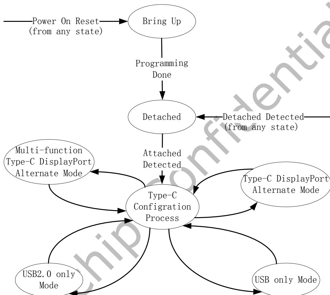
Fig. 18-4 Type-C Subsystem Mode of Operations Flow
