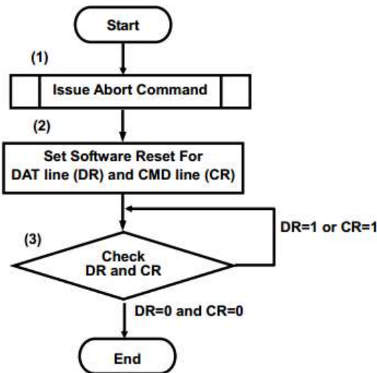
Fig. 16-13 Asynchronous Abort Sequence
