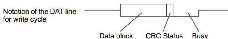
Fig. 16-22 Wait Write Transfer by Stop At Block Gap Request
