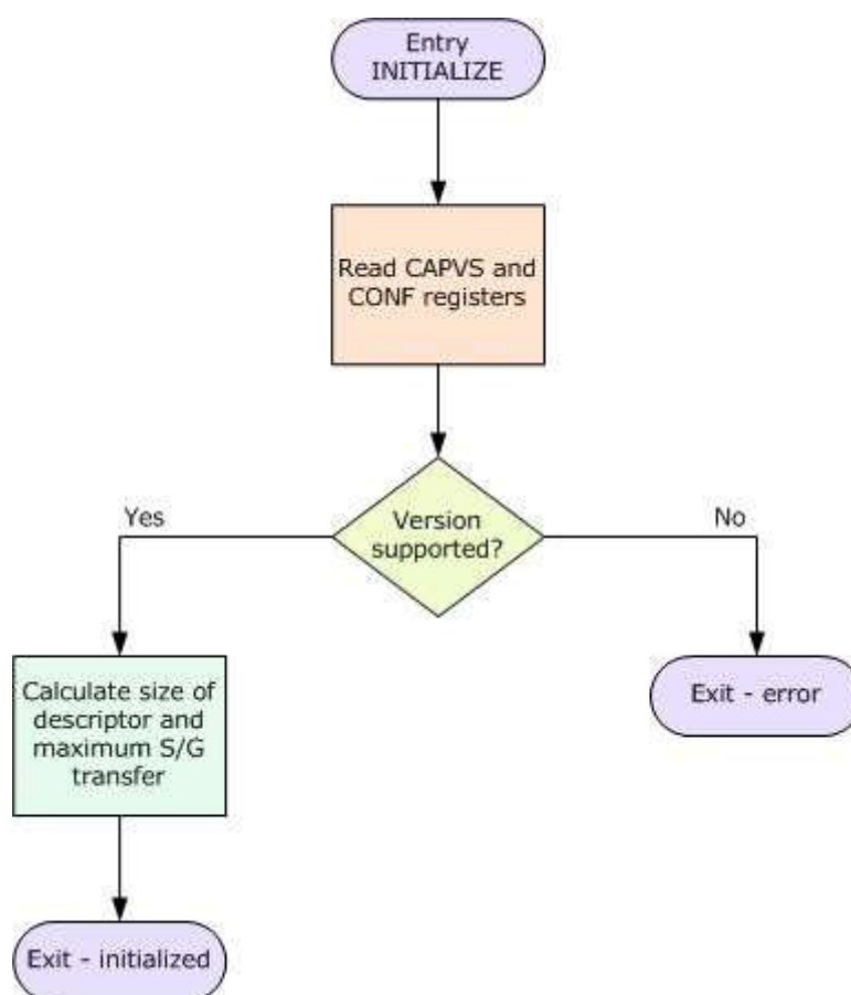
Fig. 17-23 Firmware Initialization
