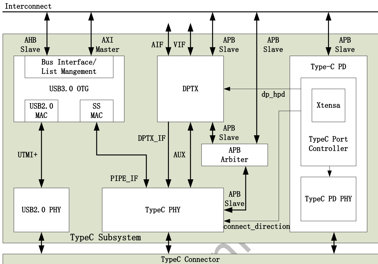
Fig. 18-1 TypeC Subsystem Block Diagram
