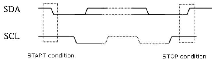
Fig. 11-3 I2C Start and stop conditions
