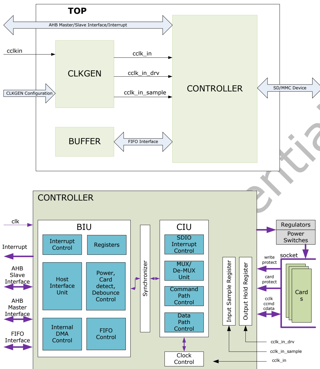
Fig. 1-1 Host Controller Block Diagram
