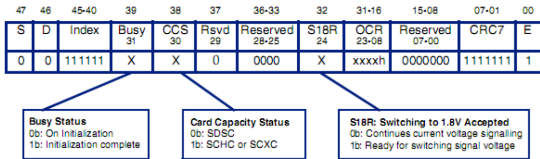
Fig. 1-14 ACMD41 Response(R3)
