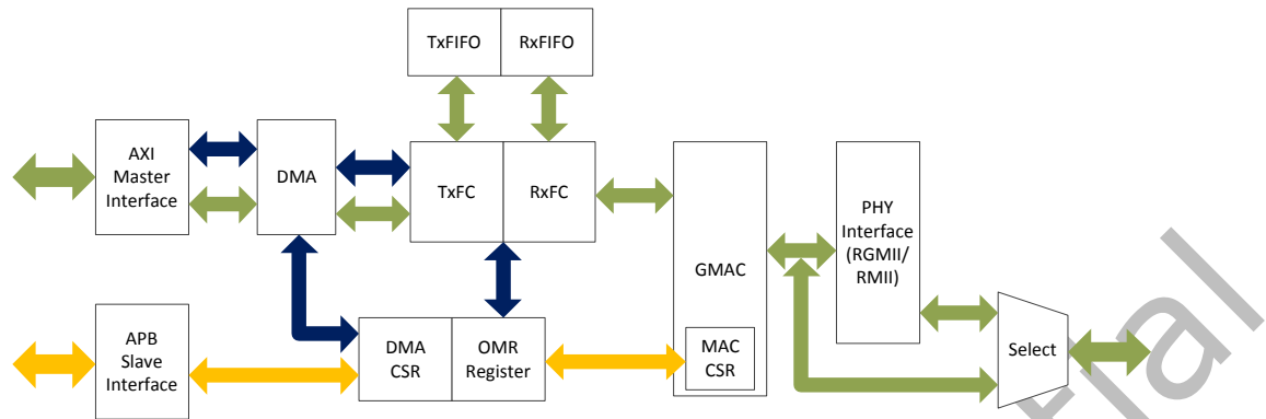
Fig. 15-1 GMAC Architecture
