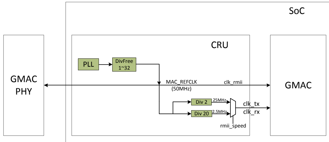
Fig. 15-12 RMII clock architecture when clock source from CRU
